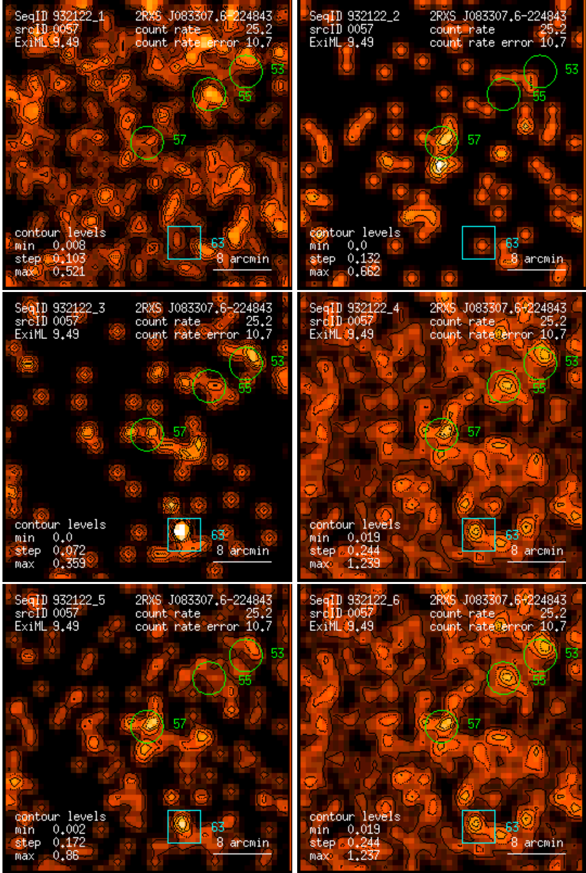
Figure 57: RASS 932122: detection 0057: band rate images, Gaussian filter: (1) PSPC channels 11 – 41, (2) 52 – 90, (3) 91 – 201, (4) 11 – 235, (5) 52 – 201, (6) 11 – 201. Broad band rates in counts/ks. Band rate contour levels in counts/ks/arcmin 2 .
