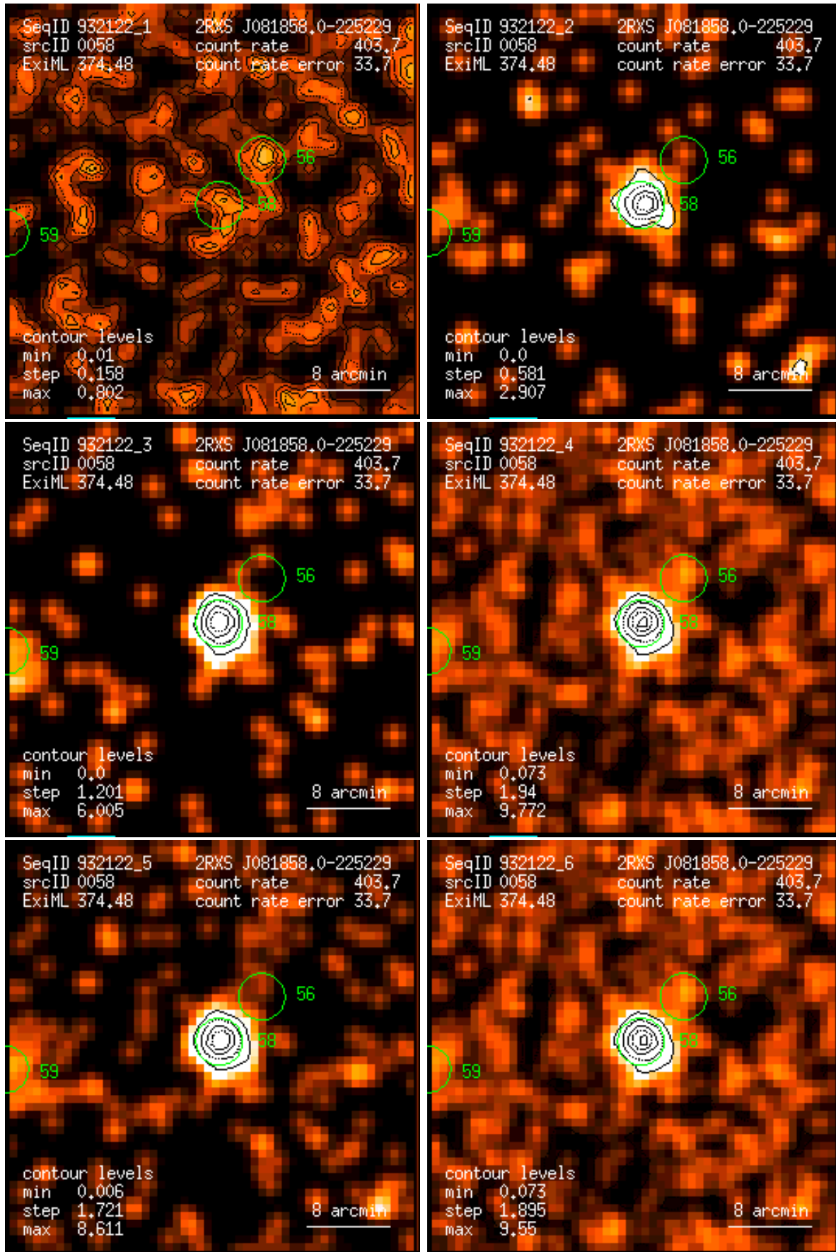
Figure 58: RASS 932122: detection 0058: band rate images, Gaussian filter: (1) PSPC channels 11 – 41, (2) 52 – 90, (3) 91 – 201, (4) 11 – 235, (5) 52 – 201, (6) 11 – 201. Broad band rates in counts/ks. Band rate contour levels in counts/ks/arcmin 2 .
