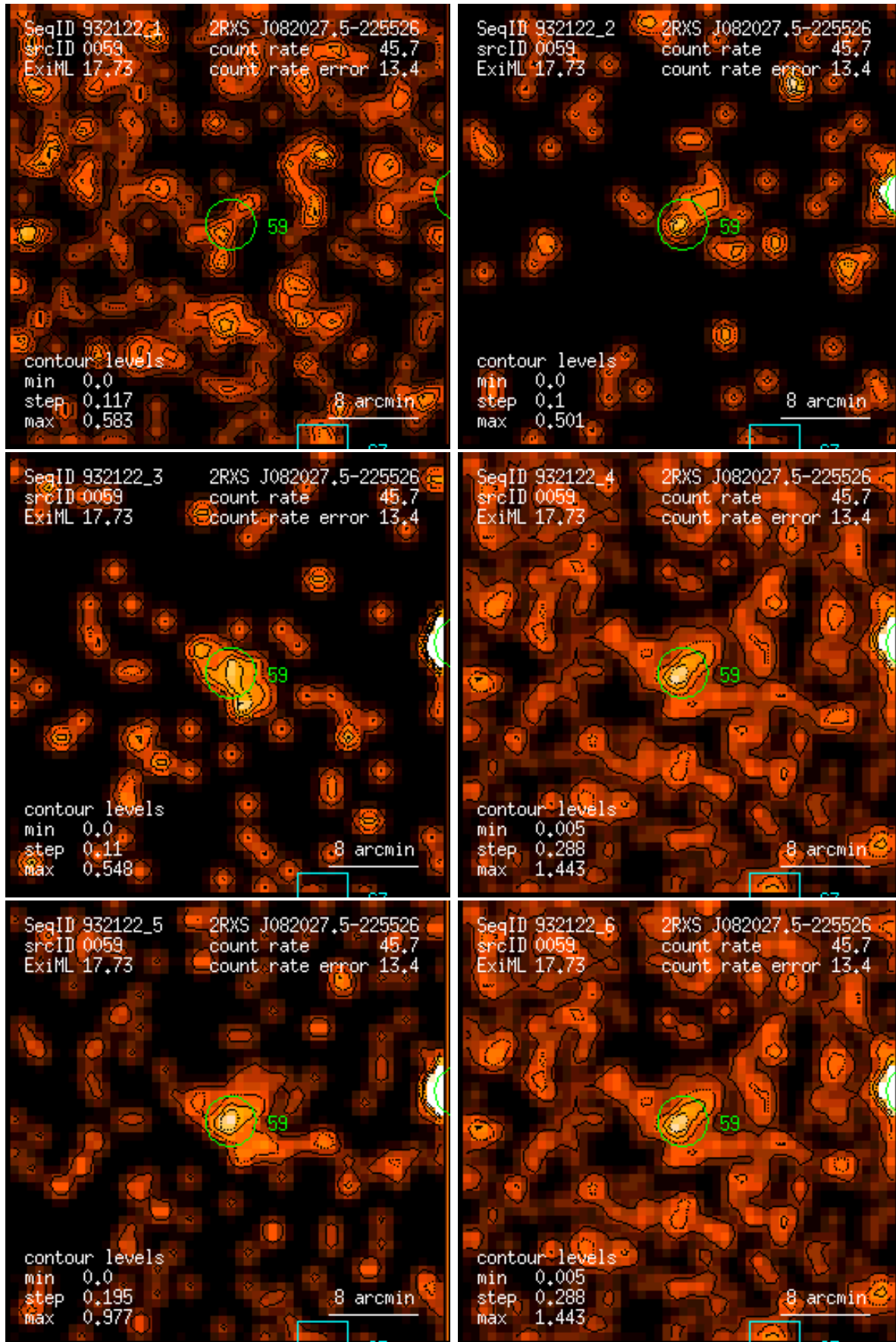
Figure 59: RASS 932122: detection 0059: band rate images, Gaussian filter: (1) PSPC channels 11 – 41, (2) 52 – 90, (3) 91 – 201, (4) 11 – 235, (5) 52 – 201, (6) 11 – 201. Broad band rates in counts/ks. Band rate contour levels in counts/ks/arcmin 2 .
