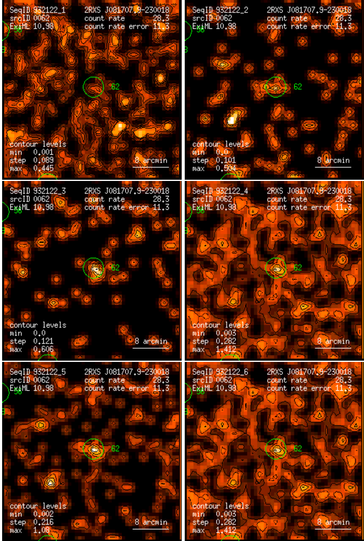
Figure 62: RASS 932122: detection 0062: band rate images, Gaussian filter: (1) PSPC channels 11 – 41, (2) 52 – 90, (3) 91 – 201, (4) 11 – 235, (5) 52 – 201, (6) 11 – 201. Broad band rates in counts/ks. Band rate contour levels in counts/ks/arcmin 2 .
