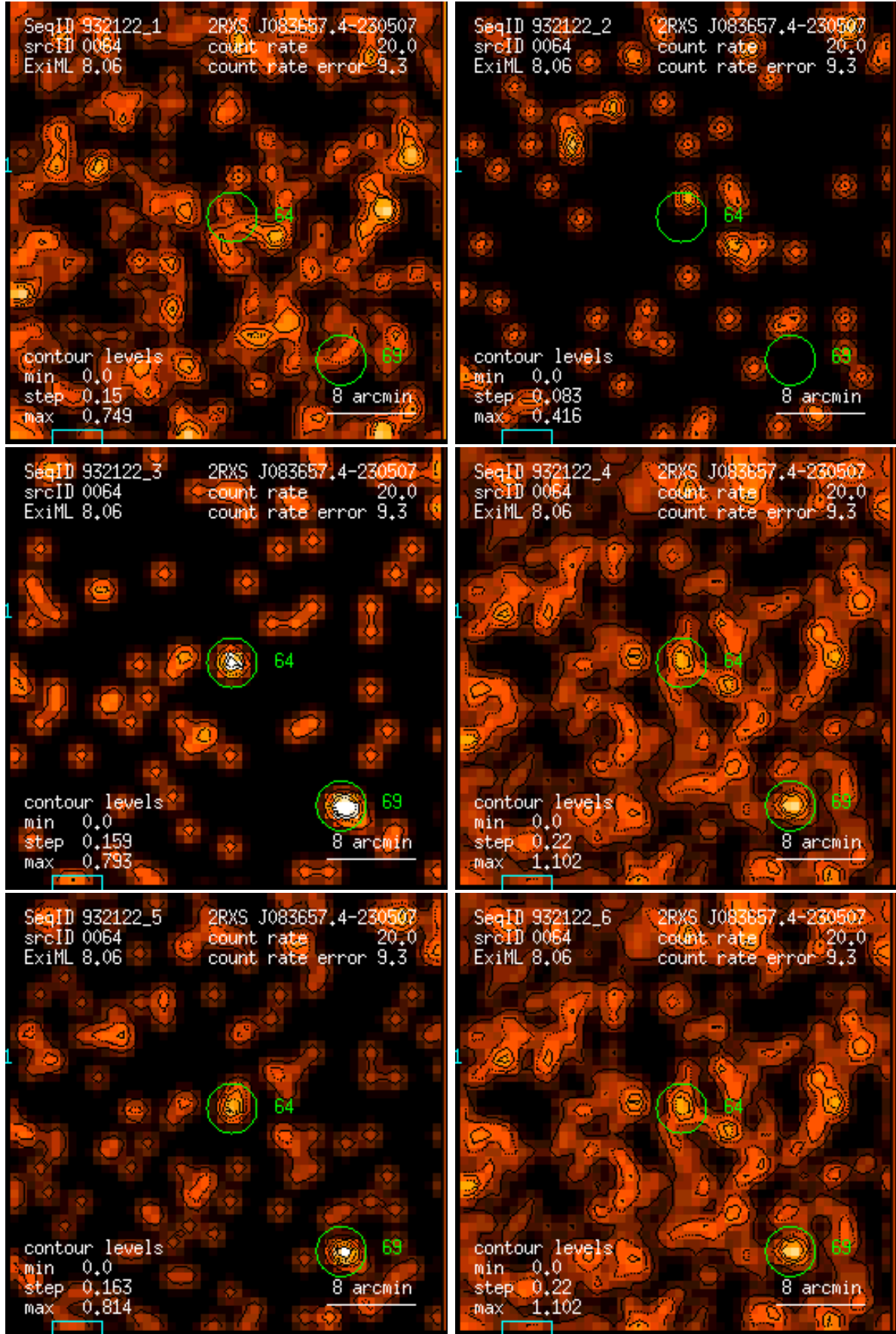
Figure 64: RASS 932122: detection 0064: band rate images, Gaussian filter: (1) PSPC channels 11 – 41, (2) 52 – 90, (3) 91 – 201, (4) 11 – 235, (5) 52 – 201, (6) 11 – 201. Broad band rates in counts/ks. Band rate contour levels in counts/ks/arcmin 2 .
