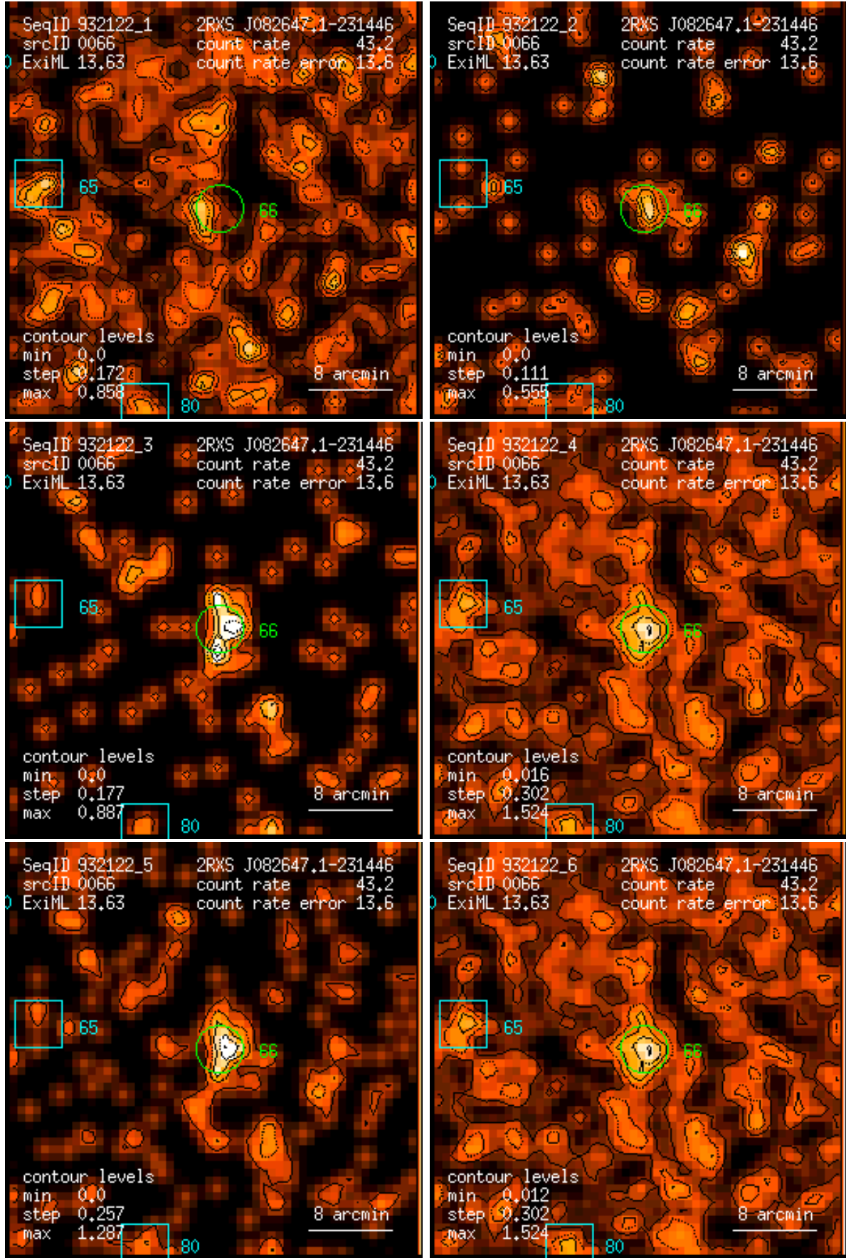
Figure 66: RASS 932122: detection 0066: band rate images, Gaussian filter: (1) PSPC channels 11 – 41, (2) 52 – 90, (3) 91 – 201, (4) 11 – 235, (5) 52 – 201, (6) 11 – 201. Broad band rates in counts/ks. Band rate contour levels in counts/ks/arcmin 2 .
