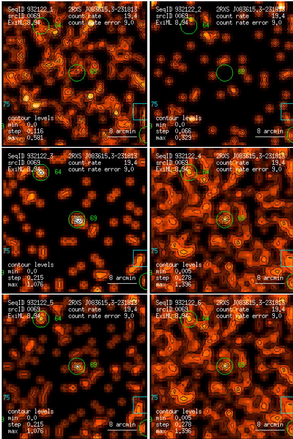
Figure 69: RASS 932122: detection 0069: band rate images, Gaussian filter: (1) PSPC channels 11 – 41, (2) 52 – 90, (3) 91 – 201, (4) 11 – 235, (5) 52 – 201, (6) 11 – 201. Broad band rates in counts/ks. Band rate contour levels in counts/ks/arcmin 2 .
