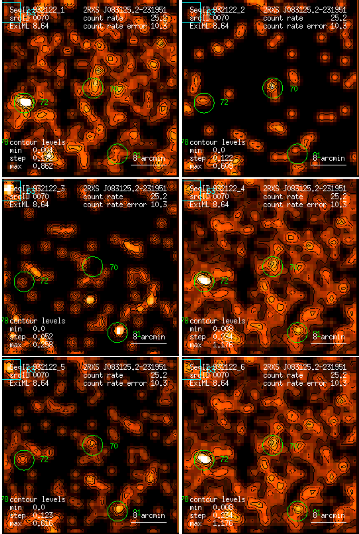
Figure 70: RASS 932122: detection 0070: band rate images, Gaussian filter: (1) PSPC channels 11 – 41, (2) 52 – 90, (3) 91 – 201, (4) 11 – 235, (5) 52 – 201, (6) 11 – 201. Broad band rates in counts/ks. Band rate contour levels in counts/ks/arcmin 2 .
