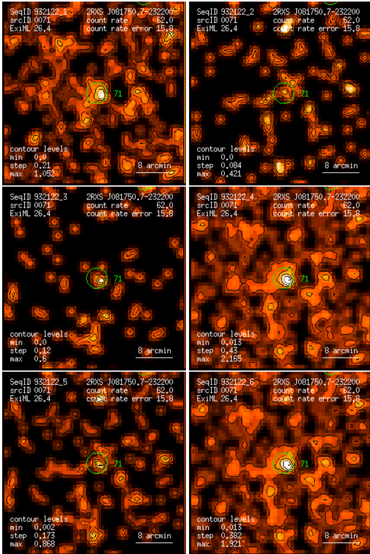
Figure 71: RASS 932122: detection 0071: band rate images, Gaussian filter: (1) PSPC channels 11 – 41, (2) 52 – 90, (3) 91 – 201, (4) 11 – 235, (5) 52 – 201, (6) 11 – 201. Broad band rates in counts/ks. Band rate contour levels in counts/ks/arcmin 2 .
