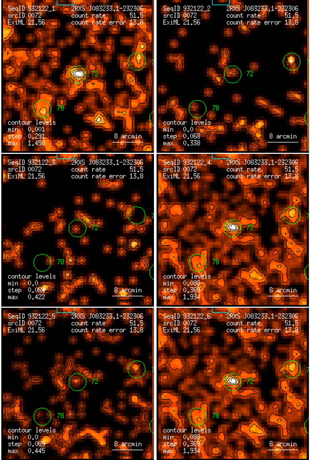
Figure 72: RASS 932122: detection 0072: band rate images, Gaussian filter: (1) PSPC channels 11 – 41, (2) 52 – 90, (3) 91 – 201, (4) 11 – 235, (5) 52 – 201, (6) 11 – 201. Broad band rates in counts/ks. Band rate contour levels in counts/ks/arcmin 2 .
