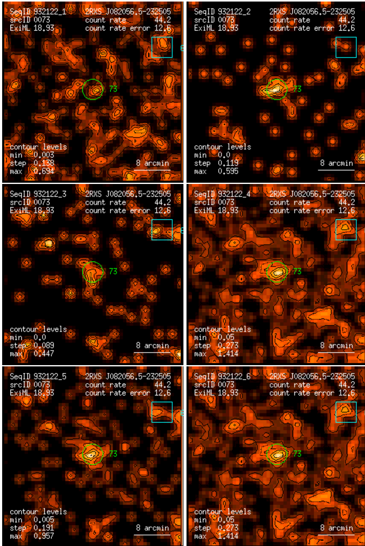
Figure 73: RASS 932122: detection 0073: band rate images, Gaussian filter: (1) PSPC channels 11 – 41, (2) 52 – 90, (3) 91 – 201, (4) 11 – 235, (5) 52 – 201, (6) 11 – 201. Broad band rates in counts/ks. Band rate contour levels in counts/ks/arcmin 2 .
