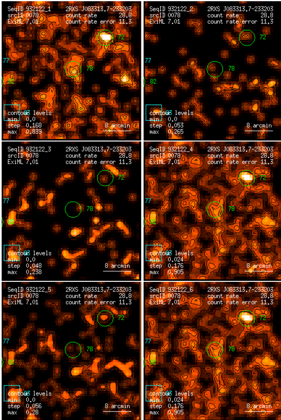
Figure 78: RASS 932122: detection 0078: band rate images, Gaussian filter: (1) PSPC channels 11 – 41, (2) 52 – 90, (3) 91 – 201, (4) 11 – 235, (5) 52 – 201, (6) 11 – 201. Broad band rates in counts/ks. Band rate contour levels in counts/ks/arcmin 2 .
