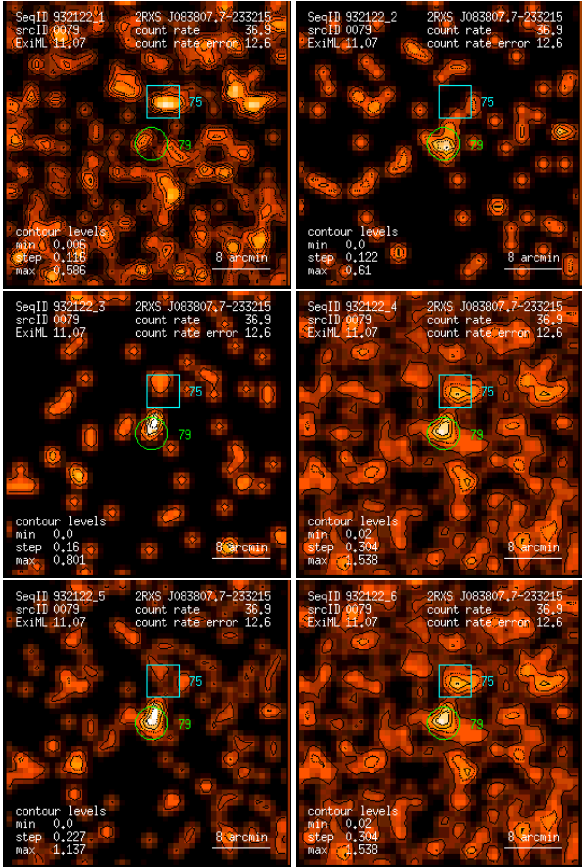
Figure 79: RASS 932122: detection 0079: band rate images, Gaussian filter: (1) PSPC channels 11 – 41, (2) 52 – 90, (3) 91 – 201, (4) 11 – 235, (5) 52 – 201, (6) 11 – 201. Broad band rates in counts/ks. Band rate contour levels in counts/ks/arcmin 2 .
