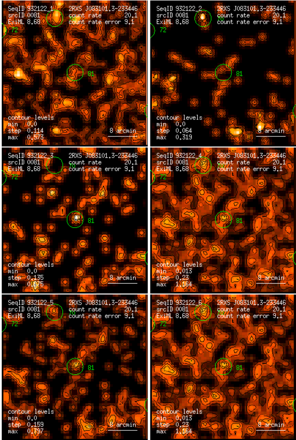
Figure 81: RASS 932122: detection 0081: band rate images, Gaussian filter: (1) PSPC channels 11 – 41, (2) 52 – 90, (3) 91 – 201, (4) 11 – 235, (5) 52 – 201, (6) 11 – 201. Broad band rates in counts/ks. Band rate contour levels in counts/ks/arcmin 2 .
