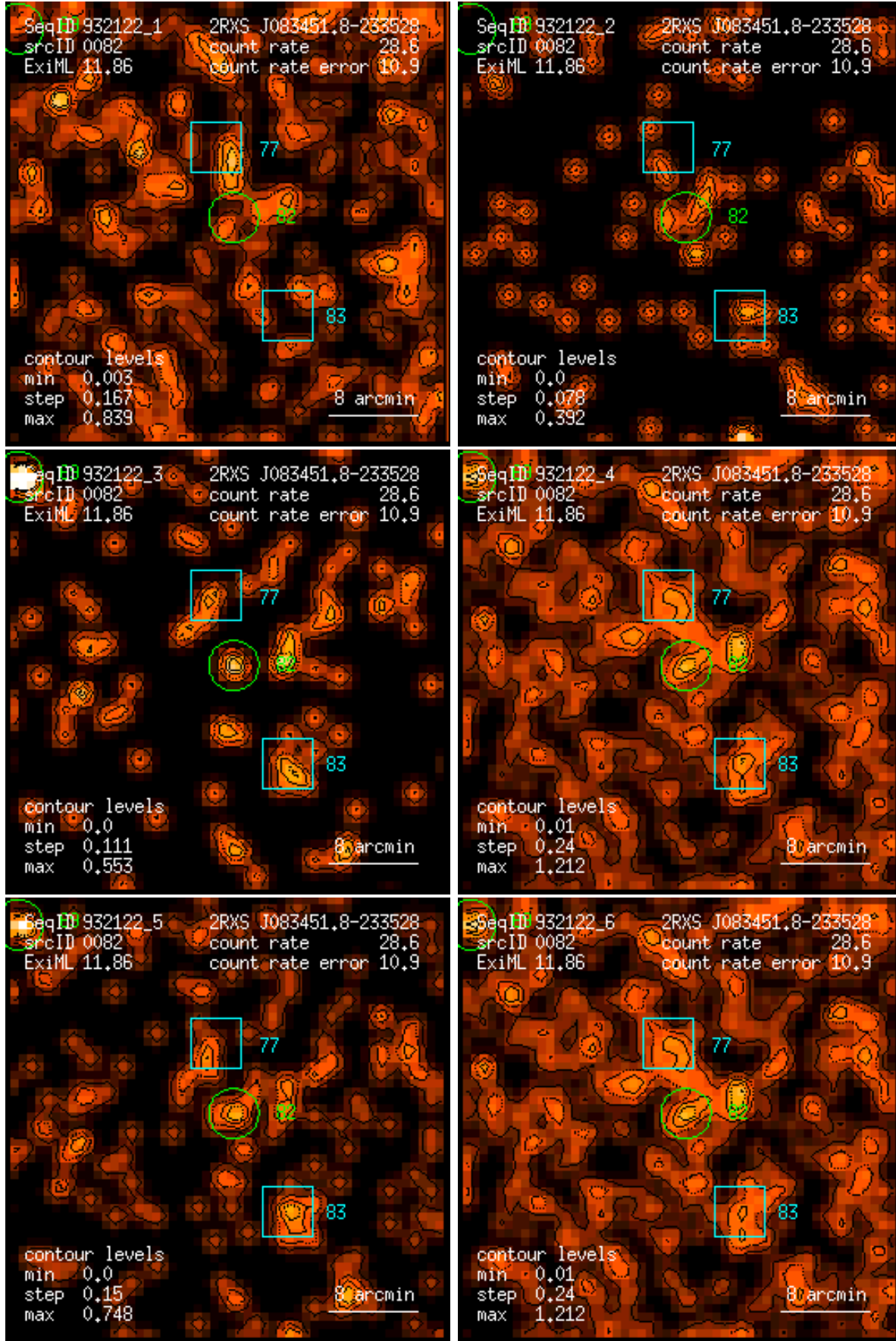
Figure 82: RASS 932122: detection 0082: band rate images, Gaussian filter: (1) PSPC channels 11 – 41, (2) 52 – 90, (3) 91 – 201, (4) 11 – 235, (5) 52 – 201, (6) 11 – 201. Broad band rates in counts/ks. Band rate contour levels in counts/ks/arcmin 2 .
