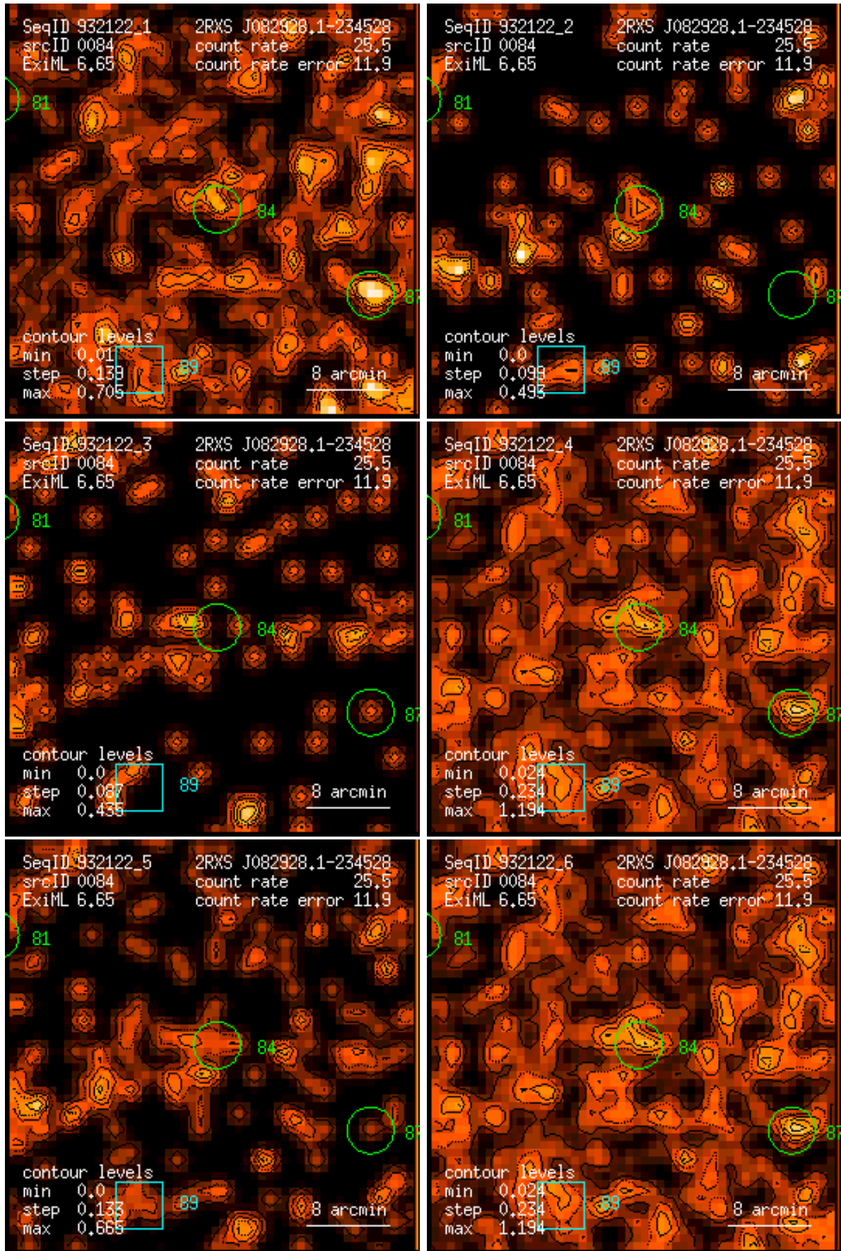
Figure 84: RASS 932122: detection 0084: band rate images, Gaussian filter: (1) PSPC channels 11 – 41, (2) 52 – 90, (3) 91 – 201, (4) 11 – 235, (5) 52 – 201, (6) 11 – 201. Broad band rates in counts/ks. Band rate contour levels in counts/ks/arcmin 2 .
