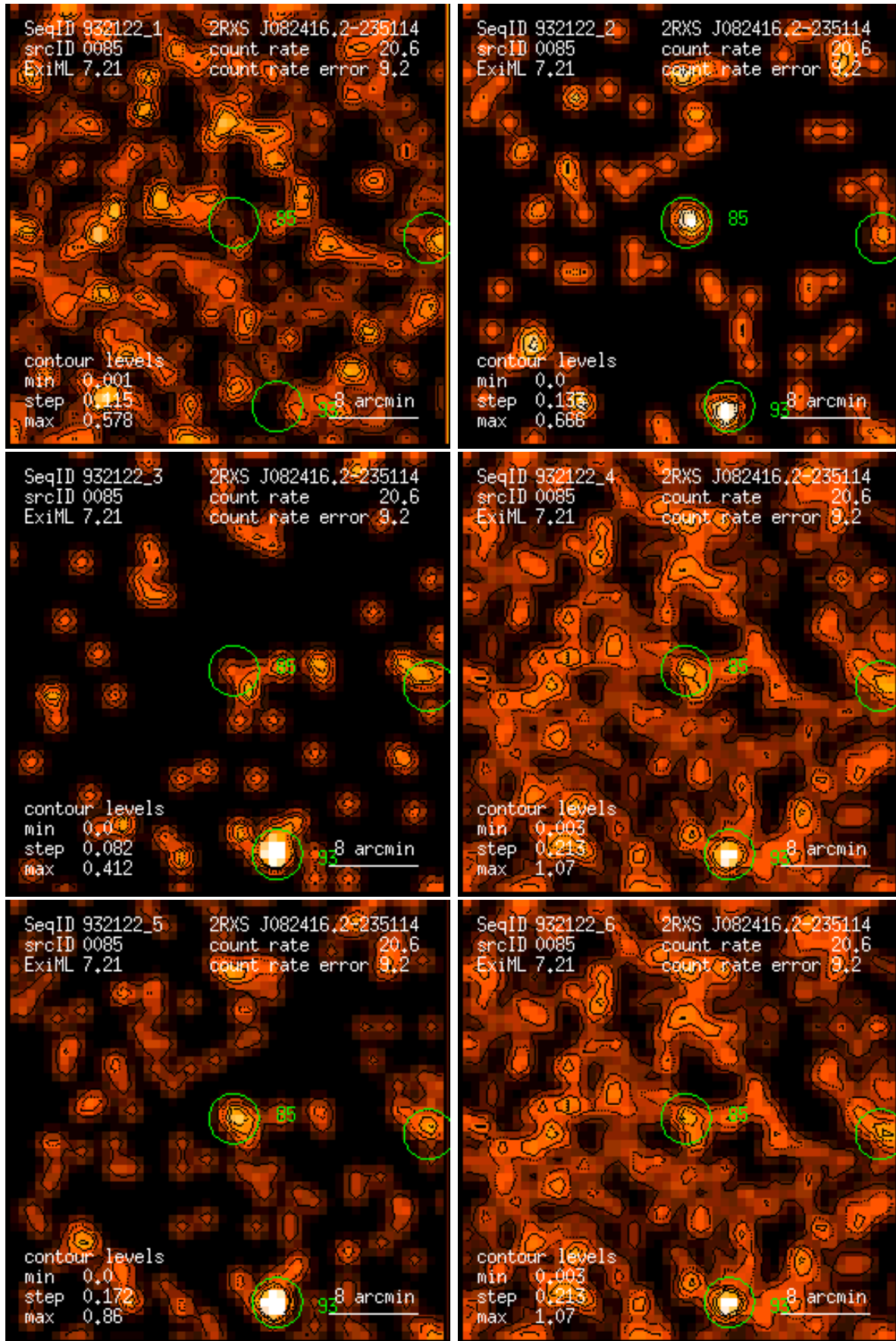
Figure 85: RASS 932122: detection 0085: band rate images, Gaussian filter: (1) PSPC channels 11 – 41, (2) 52 – 90, (3) 91 – 201, (4) 11 – 235, (5) 52 – 201, (6) 11 – 201. Broad band rates in counts/ks. Band rate contour levels in counts/ks/arcmin 2 .
