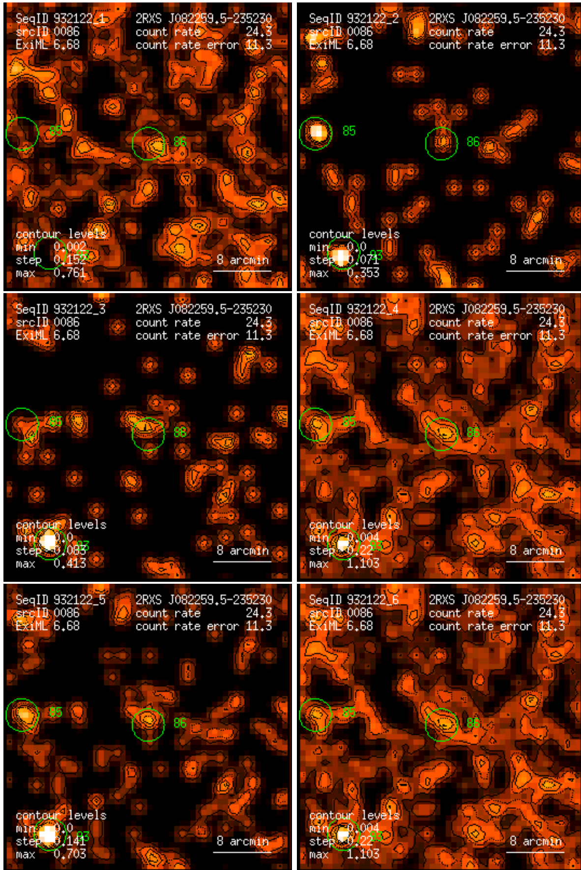
Figure 86: RASS 932122: detection 0086: band rate images, Gaussian filter: (1) PSPC channels 11 – 41, (2) 52 – 90, (3) 91 – 201, (4) 11 – 235, (5) 52 – 201, (6) 11 – 201. Broad band rates in counts/ks. Band rate contour levels in counts/ks/arcmin 2 .
