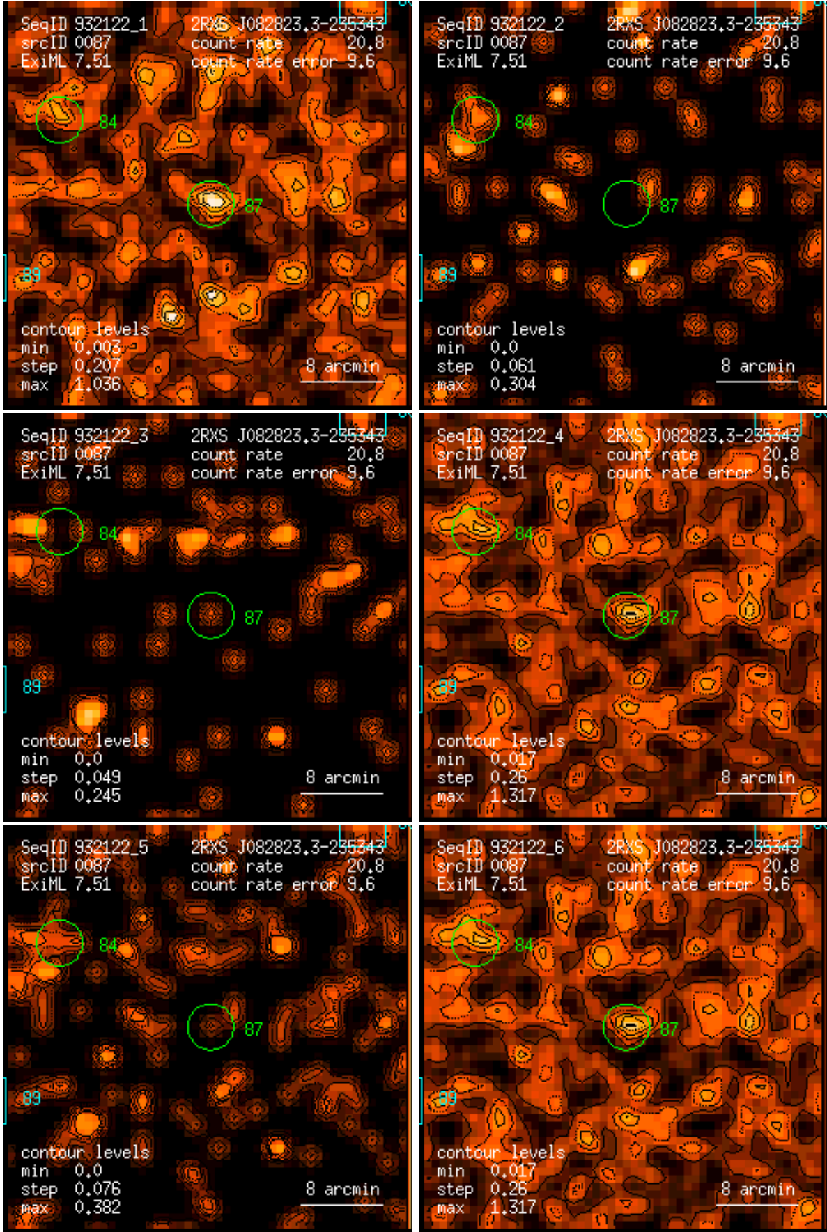
Figure 87: RASS 932122: detection 0087: band rate images, Gaussian filter: (1) PSPC channels 11 – 41, (2) 52 – 90, (3) 91 – 201, (4) 11 – 235, (5) 52 – 201, (6) 11 – 201. Broad band rates in counts/ks. Band rate contour levels in counts/ks/arcmin 2 .
