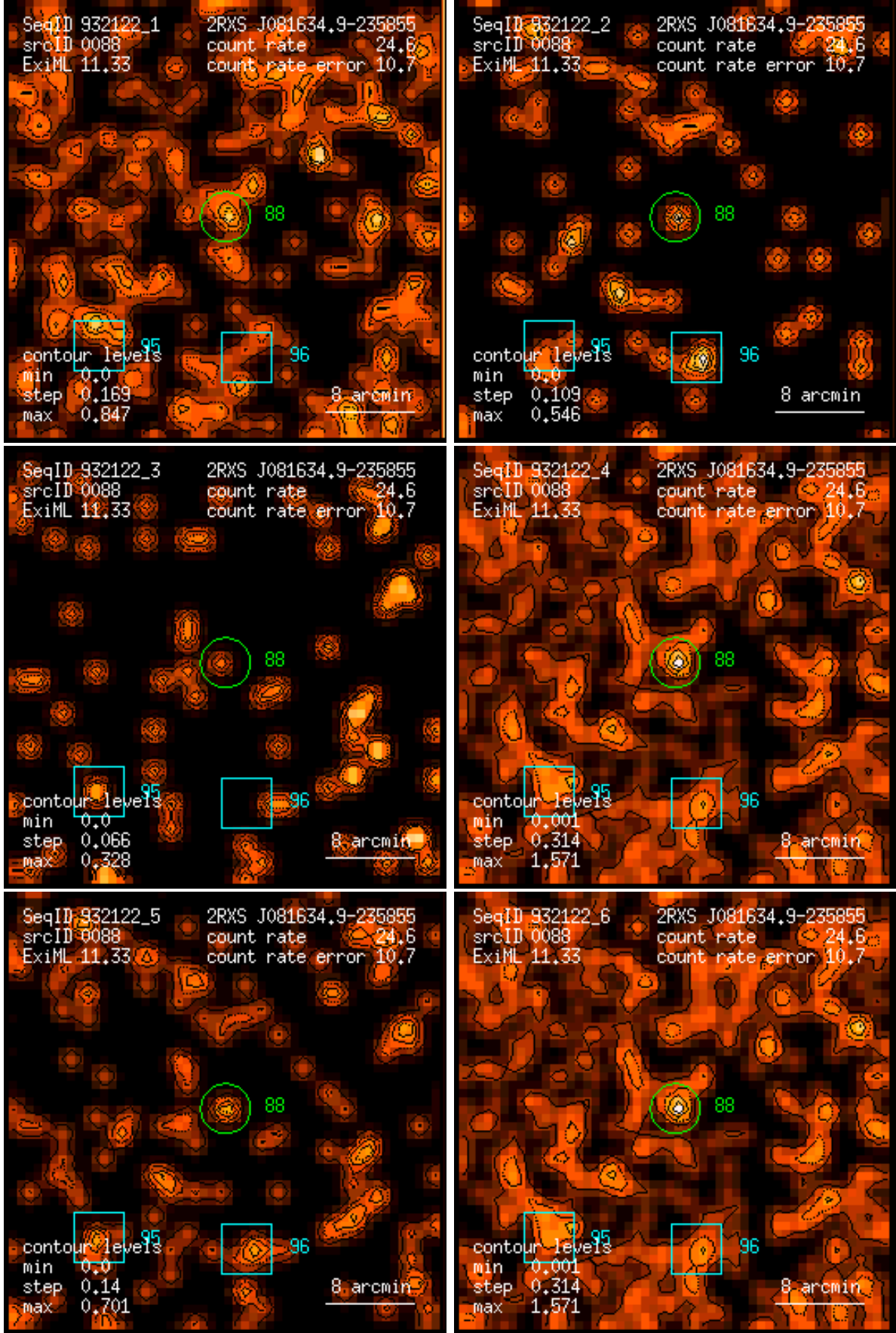
Figure 88: RASS 932122: detection 0088: band rate images, Gaussian filter: (1) PSPC channels 11 – 41, (2) 52 – 90, (3) 91 – 201, (4) 11 – 235, (5) 52 – 201, (6) 11 – 201. Broad band rates in counts/ks. Band rate contour levels in counts/ks/arcmin 2 .
