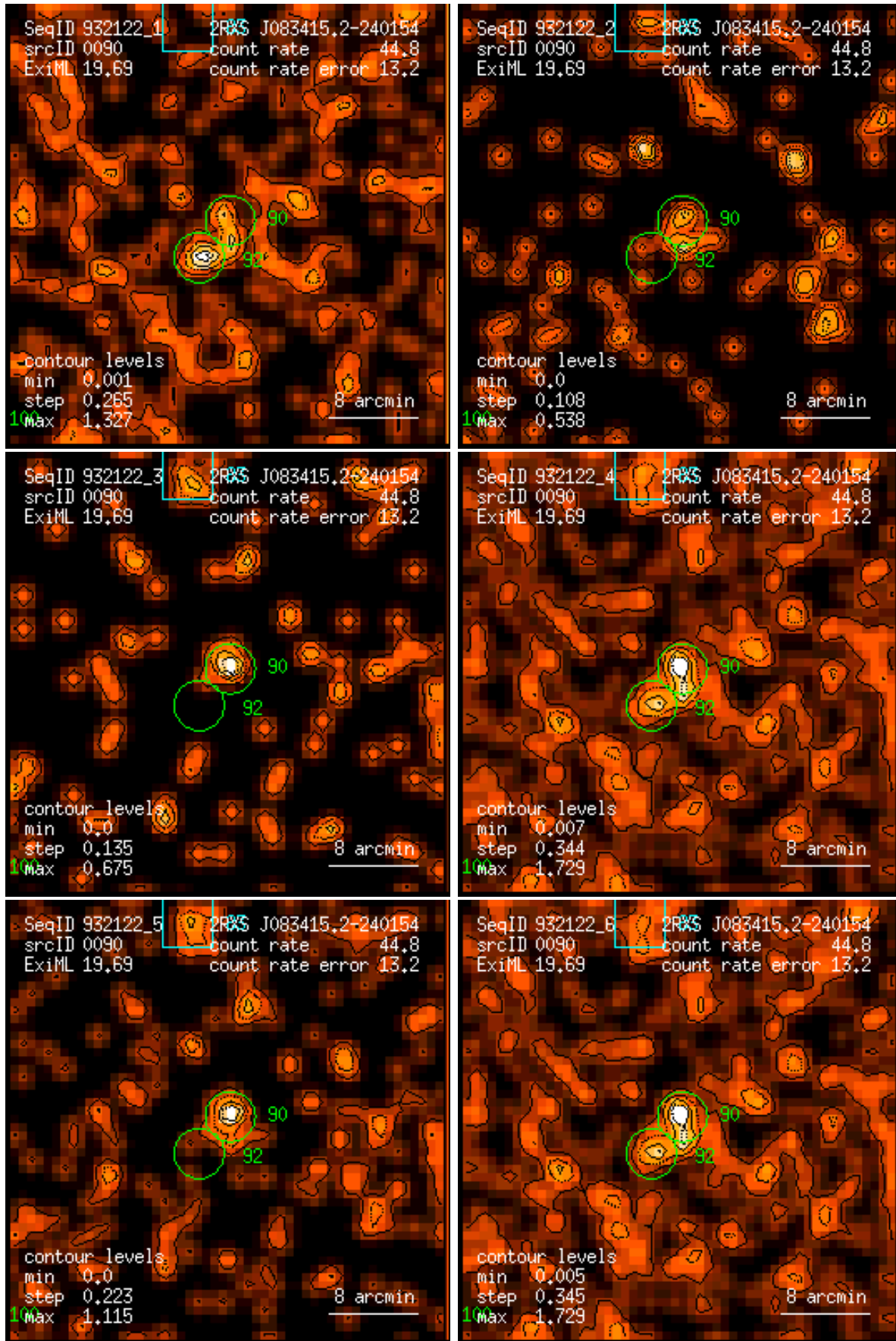
Figure 90: RASS 932122: detection 0090: band rate images, Gaussian filter: (1) PSPC channels 11 – 41, (2) 52 – 90, (3) 91 – 201, (4) 11 – 235, (5) 52 – 201, (6) 11 – 201. Broad band rates in counts/ks. Band rate contour levels in counts/ks/arcmin 2 .
