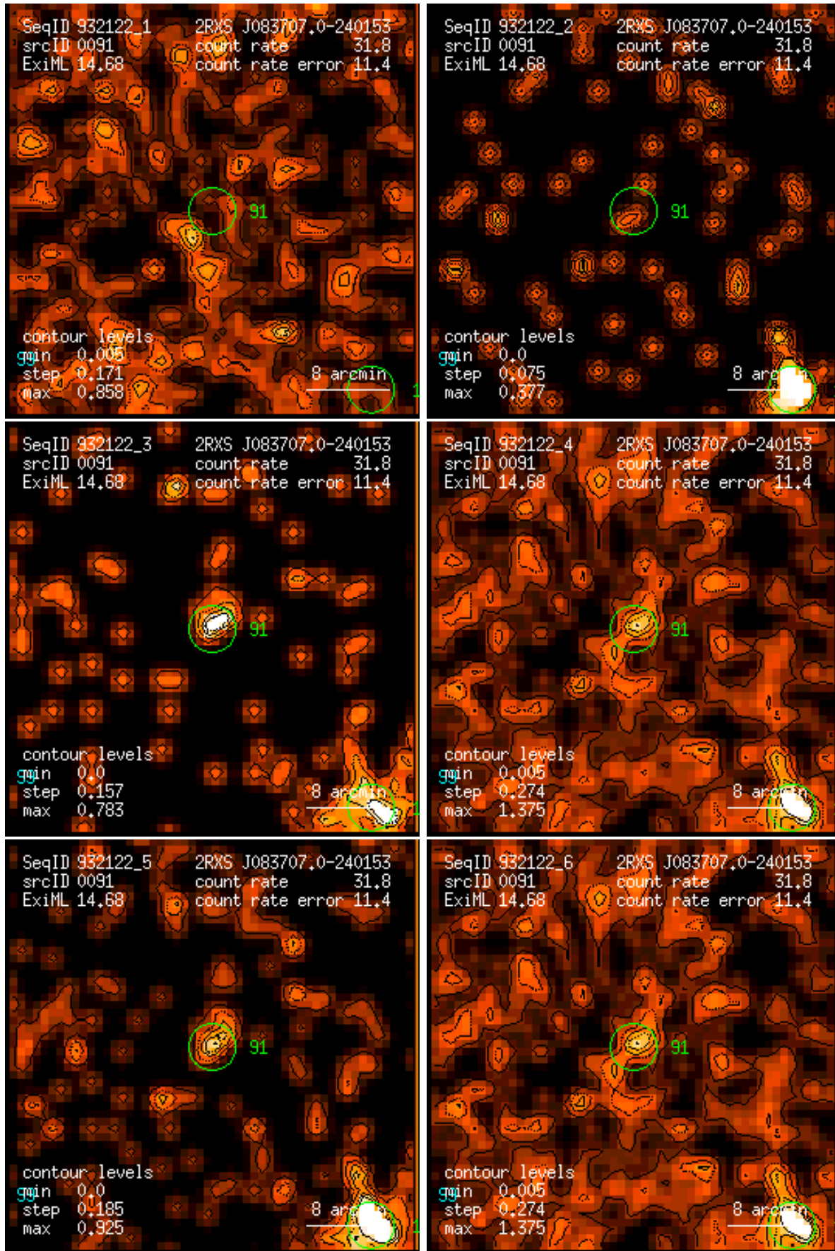
Figure 91: RASS 932122: detection 0091: band rate images, Gaussian filter: (1) PSPC channels 11 – 41, (2) 52 – 90, (3) 91 – 201, (4) 11 – 235, (5) 52 – 201, (6) 11 – 201. Broad band rates in counts/ks. Band rate contour levels in counts/ks/arcmin 2 .
