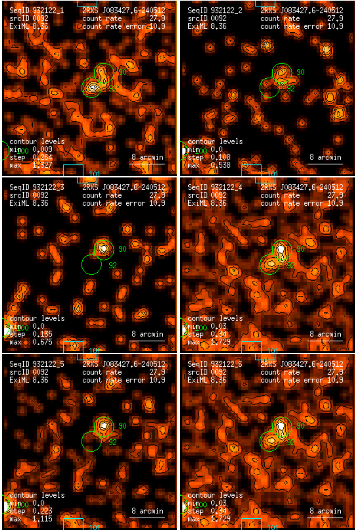
Figure 92: RASS 932122: detection 0092: band rate images, Gaussian filter: (1) PSPC channels 11 – 41, (2) 52 – 90, (3) 91 – 201, (4) 11 – 235, (5) 52 – 201, (6) 11 – 201. Broad band rates in counts/ks. Band rate contour levels in counts/ks/arcmin 2 .
