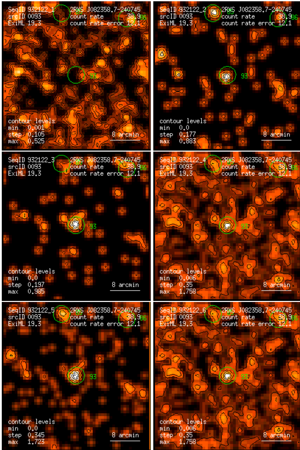
Figure 93: RASS 932122: detection 0093: band rate images, Gaussian filter: (1) PSPC channels 11 – 41, (2) 52 – 90, (3) 91 – 201, (4) 11 – 235, (5) 52 – 201, (6) 11 – 201. Broad band rates in counts/ks. Band rate contour levels in counts/ks/arcmin 2 .
