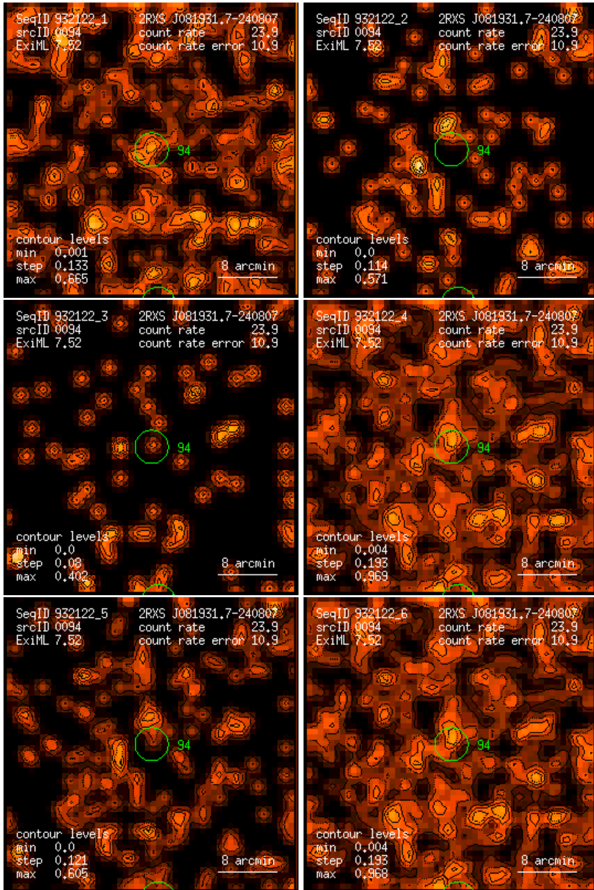
Figure 94: RASS 932122: detection 0094: band rate images, Gaussian filter: (1) PSPC channels 11 – 41, (2) 52 – 90, (3) 91 – 201, (4) 11 – 235, (5) 52 – 201, (6) 11 – 201. Broad band rates in counts/ks. Band rate contour levels in counts/ks/arcmin 2 .
