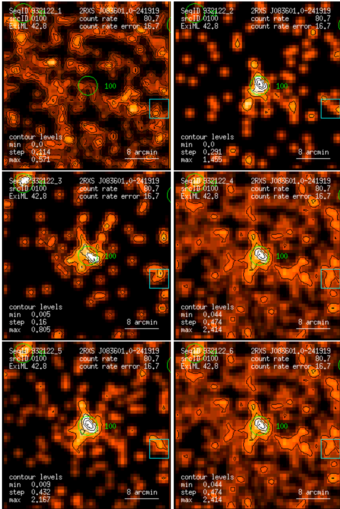
Figure 100: RASS 932122: detection 0100: band rate images, Gaussian filter: (1) PSPC channels 11 – 41, (2) 52 – 90, (3) 91 – 201, (4) 11 – 235, (5) 52 – 201, (6) 11 – 201. Broad band rates in counts/ks. Band rate contour levels in counts/ks/arcmin 2 .
