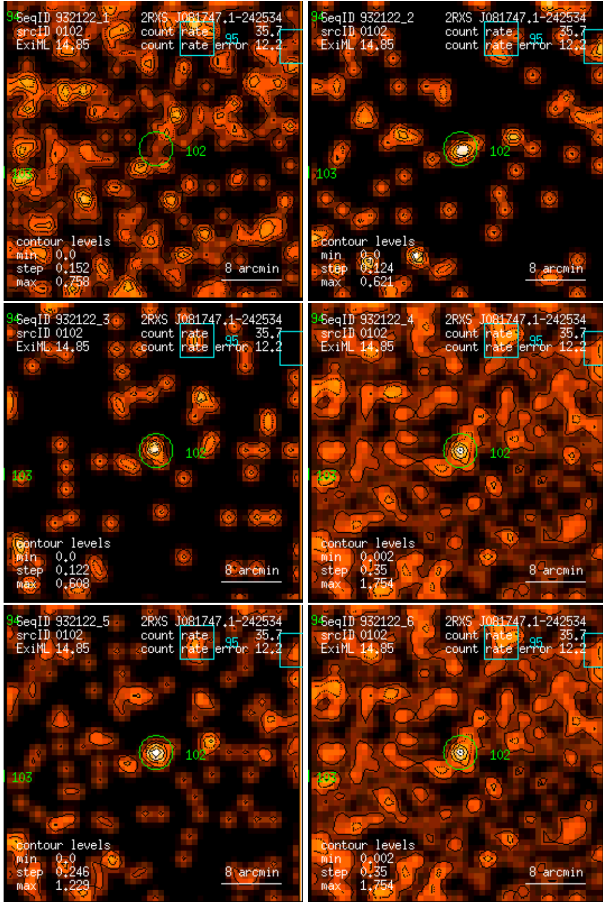
Figure 102: RASS 932122: detection 0102: band rate images, Gaussian filter: (1) PSPC channels 11 – 41, (2) 52 – 90, (3) 91 – 201, (4) 11 – 235, (5) 52 – 201, (6) 11 – 201. Broad band rates in counts/ks. Band rate contour levels in counts/ks/arcmin 2 .
