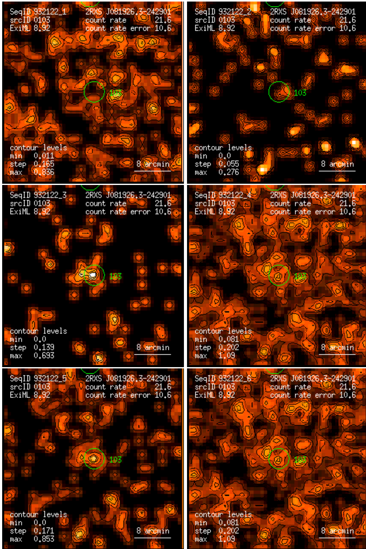
Figure 103: RASS 932122: detection 0103: band rate images, Gaussian filter: (1) PSPC channels 11 – 41, (2) 52 – 90, (3) 91 – 201, (4) 11 – 235, (5) 52 – 201, (6) 11 – 201. Broad band rates in counts/ks. Band rate contour levels in counts/ks/arcmin 2 .
