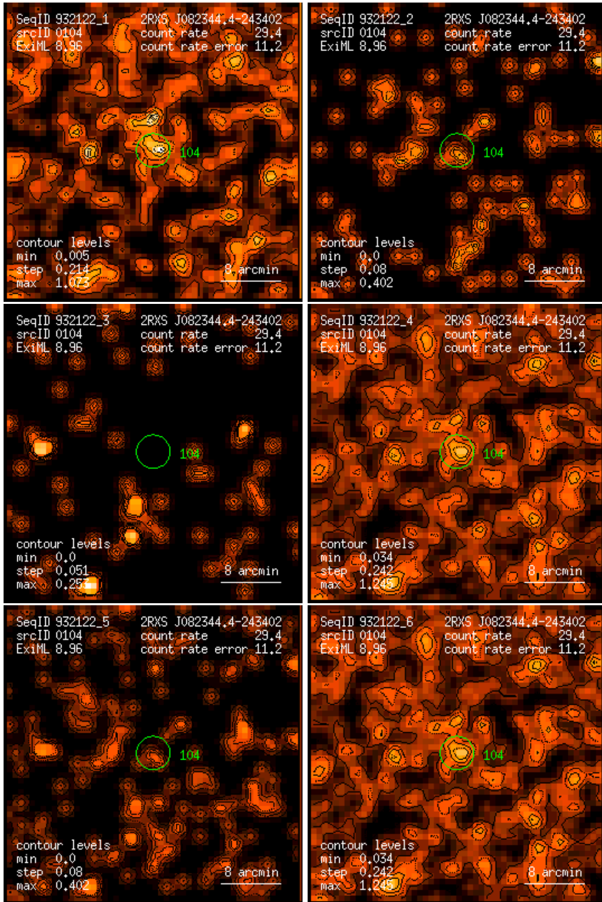
Figure 104: RASS 932122: detection 0104: band rate images, Gaussian filter: (1) PSPC channels 11 – 41, (2) 52 – 90, (3) 91 – 201, (4) 11 – 235, (5) 52 – 201, (6) 11 – 201. Broad band rates in counts/ks. Band rate contour levels in counts/ks/arcmin 2 .
