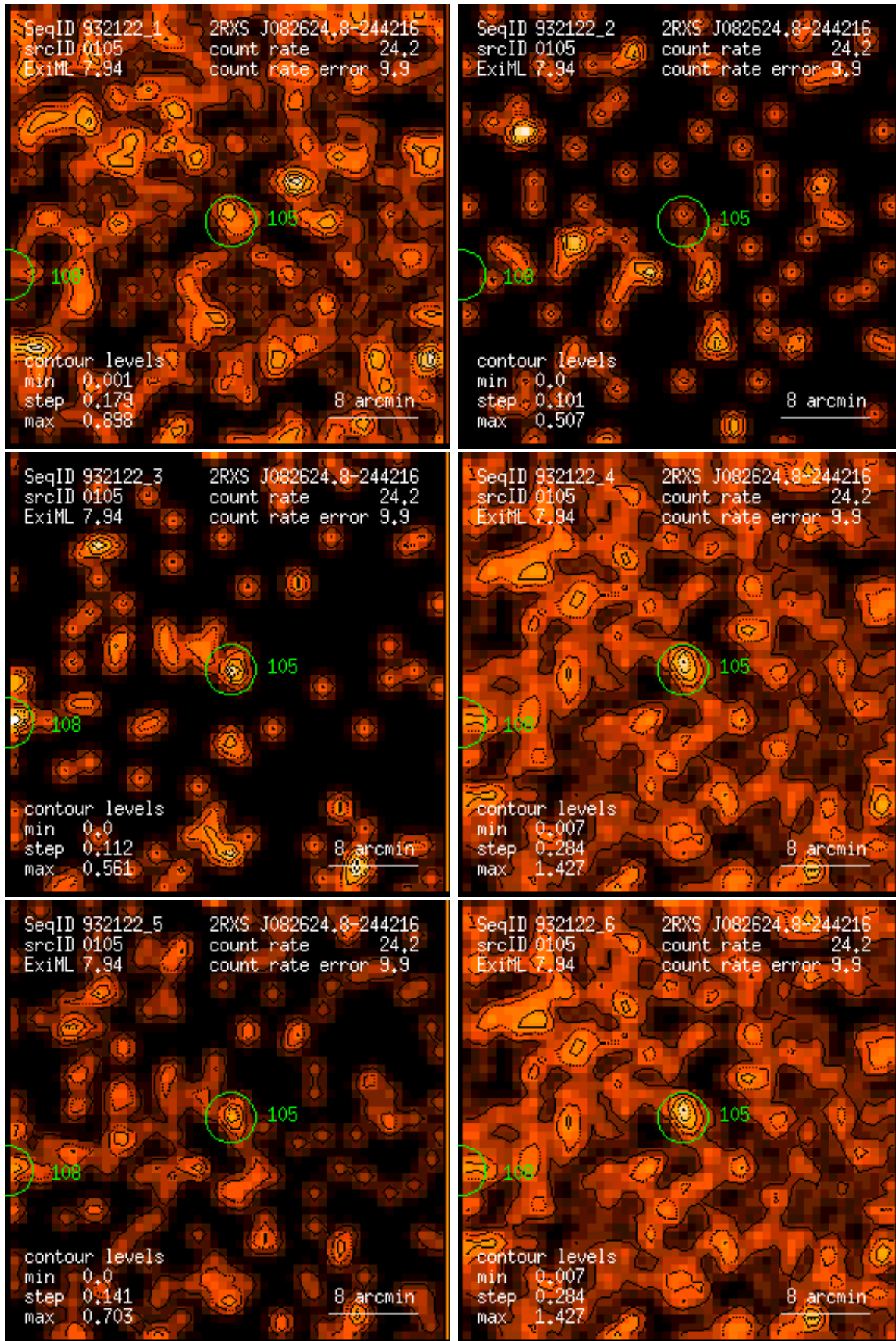
Figure 105: RASS 932122: detection 0105: band rate images, Gaussian filter: (1) PSPC channels 11 – 41, (2) 52 – 90, (3) 91 – 201, (4) 11 – 235, (5) 52 – 201, (6) 11 – 201. Broad band rates in counts/ks. Band rate contour levels in counts/ks/arcmin 2 .
