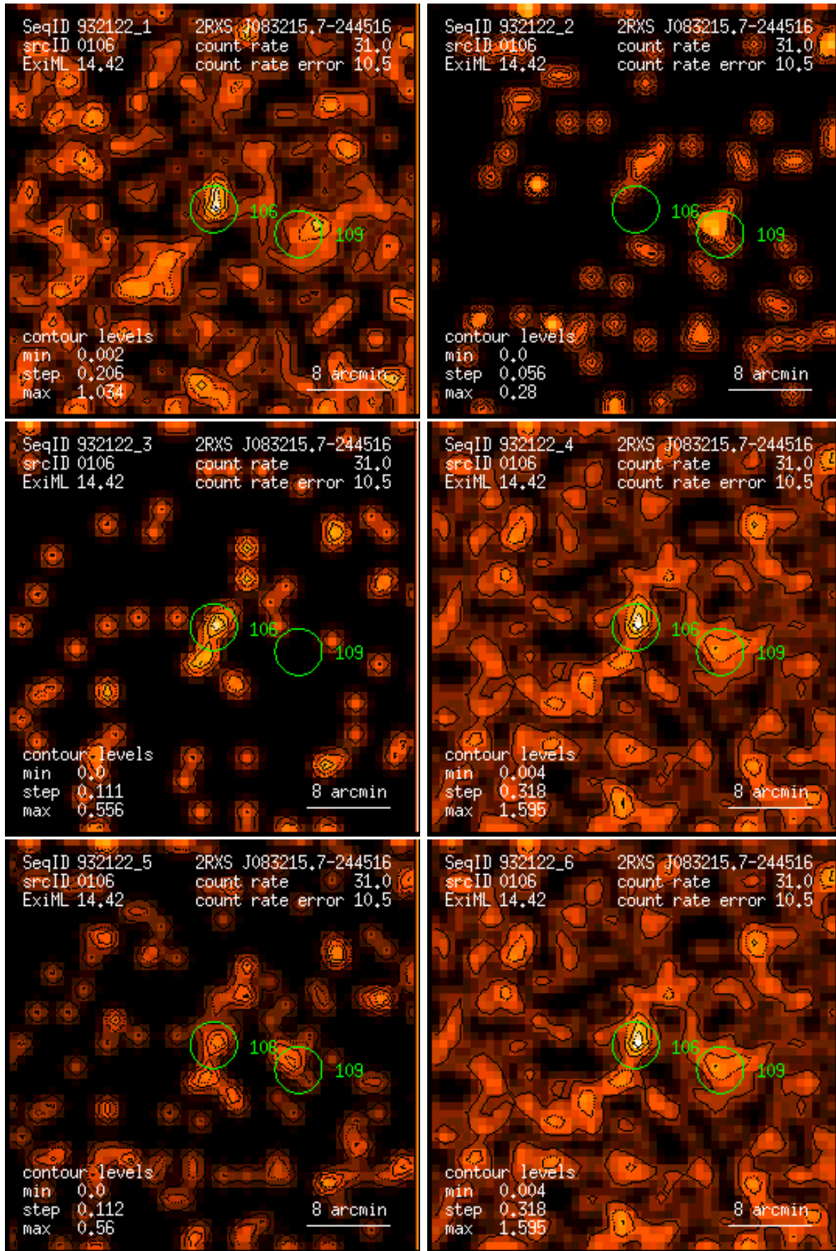
Figure 106: RASS 932122: detection 0106: band rate images, Gaussian filter: (1) PSPC channels 11 – 41, (2) 52 – 90, (3) 91 – 201, (4) 11 – 235, (5) 52 – 201, (6) 11 – 201. Broad band rates in counts/ks. Band rate contour levels in counts/ks/arcmin 2 .
