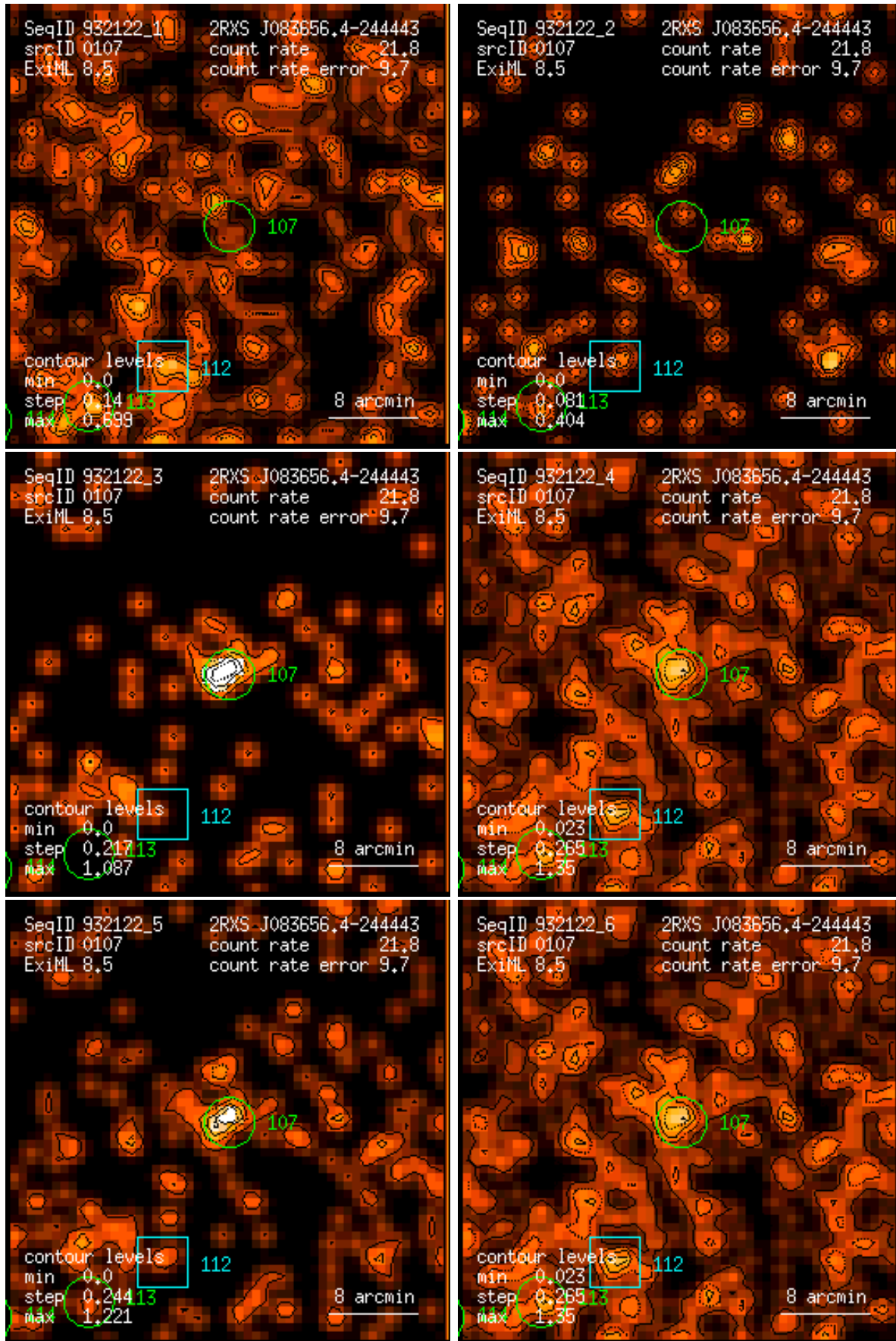
Figure 107: RASS 932122: detection 0107: band rate images, Gaussian filter: (1) PSPC channels 11 – 41, (2) 52 – 90, (3) 91 – 201, (4) 11 – 235, (5) 52 – 201, (6) 11 – 201. Broad band rates in counts/ks. Band rate contour levels in counts/ks/arcmin 2 .
