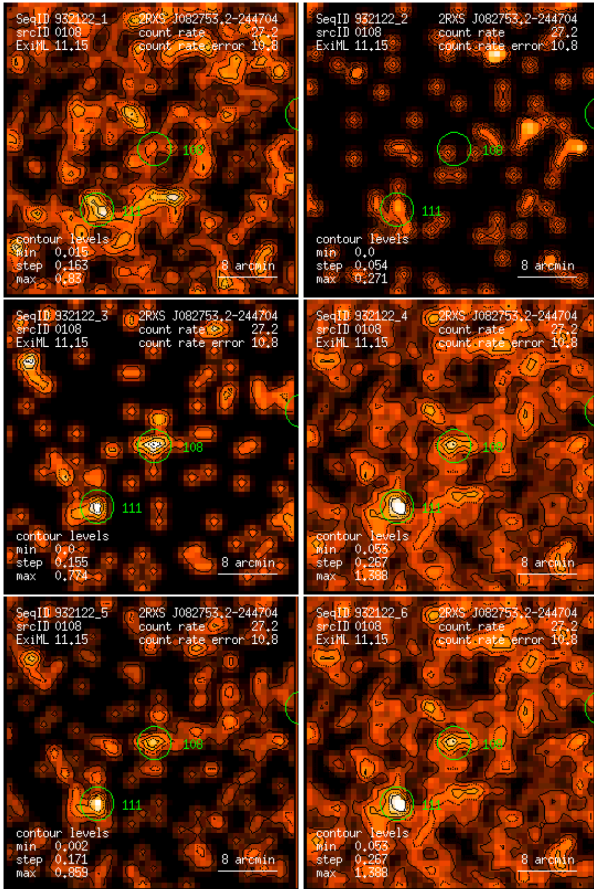
Figure 108: RASS 932122: detection 0108: band rate images, Gaussian filter: (1) PSPC channels 11 – 41, (2) 52 – 90, (3) 91 – 201, (4) 11 – 235, (5) 52 – 201, (6) 11 – 201. Broad band rates in counts/ks. Band rate contour levels in counts/ks/arcmin 2 .
