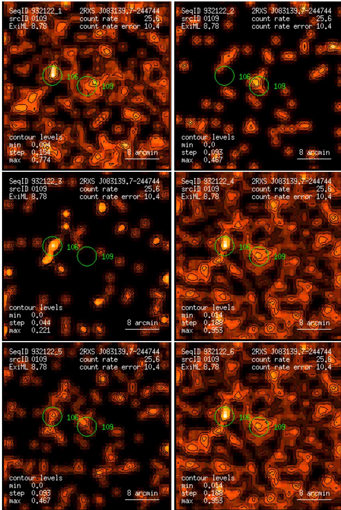
Figure 109: RASS 932122: detection 0109: band rate images, Gaussian filter: (1) PSPC channels 11 – 41, (2) 52 – 90, (3) 91 – 201, (4) 11 – 235, (5) 52 – 201, (6) 11 – 201. Broad band rates in counts/ks. Band rate contour levels in counts/ks/arcmin 2 .
