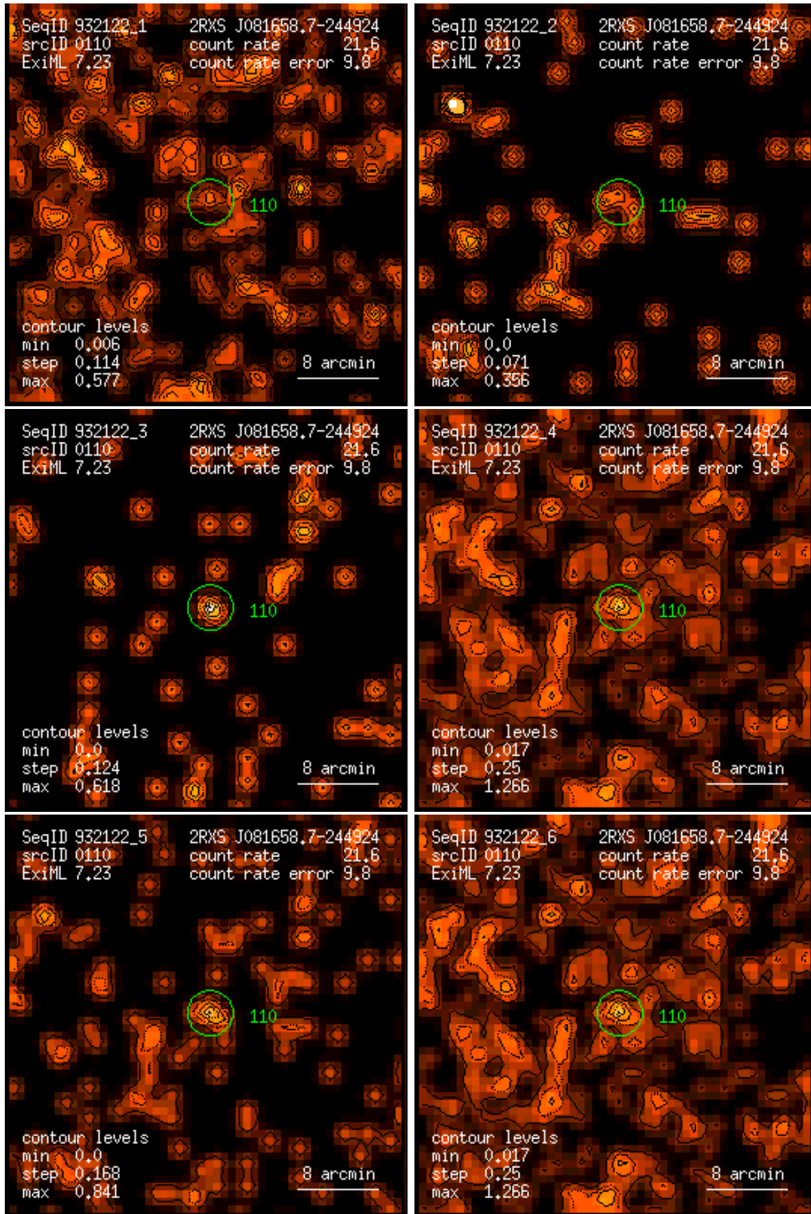
Figure 110: RASS 932122: detection 0110: band rate images, Gaussian filter: (1) PSPC channels 11 – 41, (2) 52 – 90, (3) 91 – 201, (4) 11 – 235, (5) 52 – 201, (6) 11 – 201. Broad band rates in counts/ks. Band rate contour levels in counts/ks/arcmin 2 .
