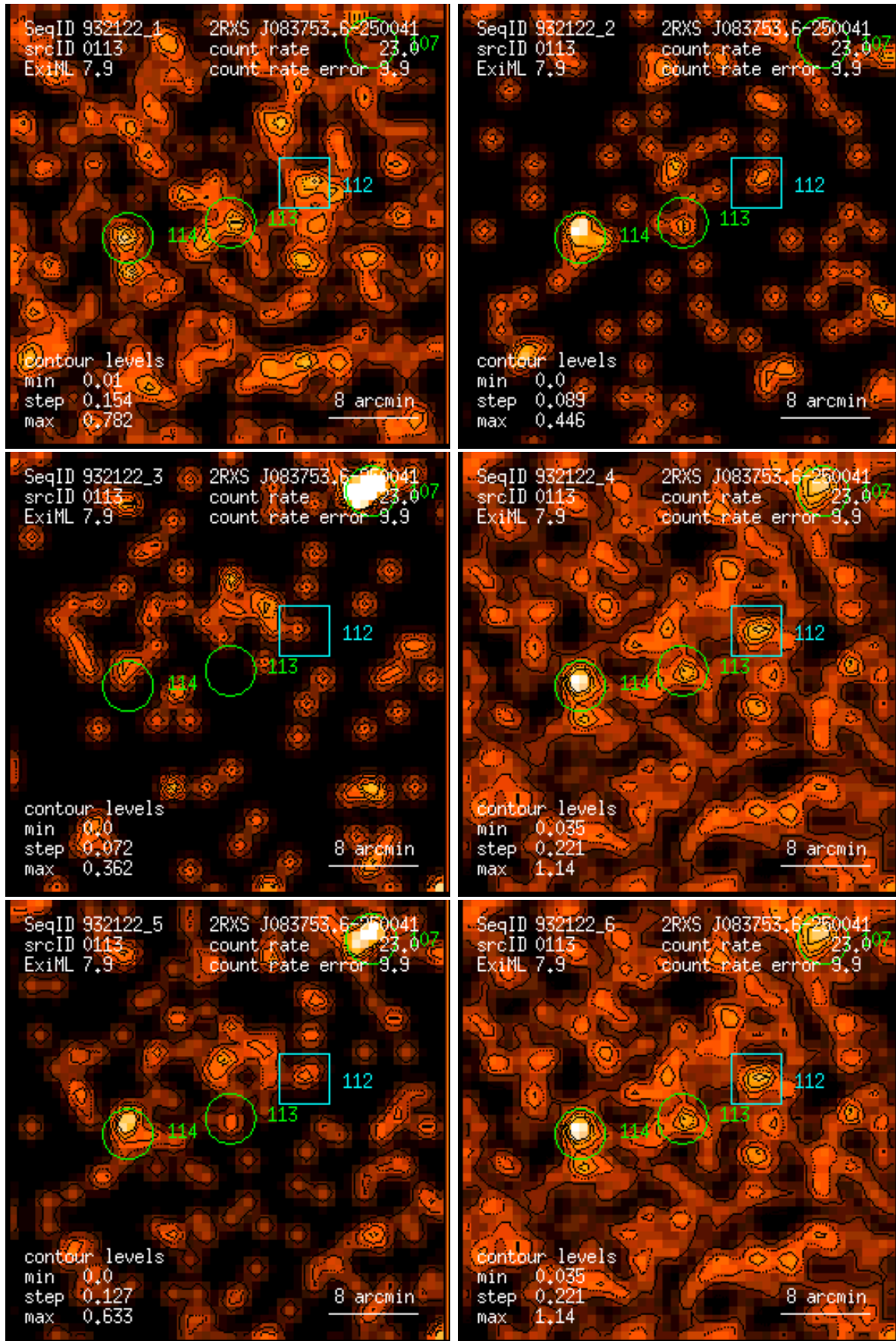
Figure 113: RASS 932122: detection 0113: band rate images, Gaussian filter: (1) PSPC channels 11 – 41, (2) 52 – 90, (3) 91 – 201, (4) 11 – 235, (5) 52 – 201, (6) 11 – 201. Broad band rates in counts/ks. Band rate contour levels in counts/ks/arcmin 2 .
