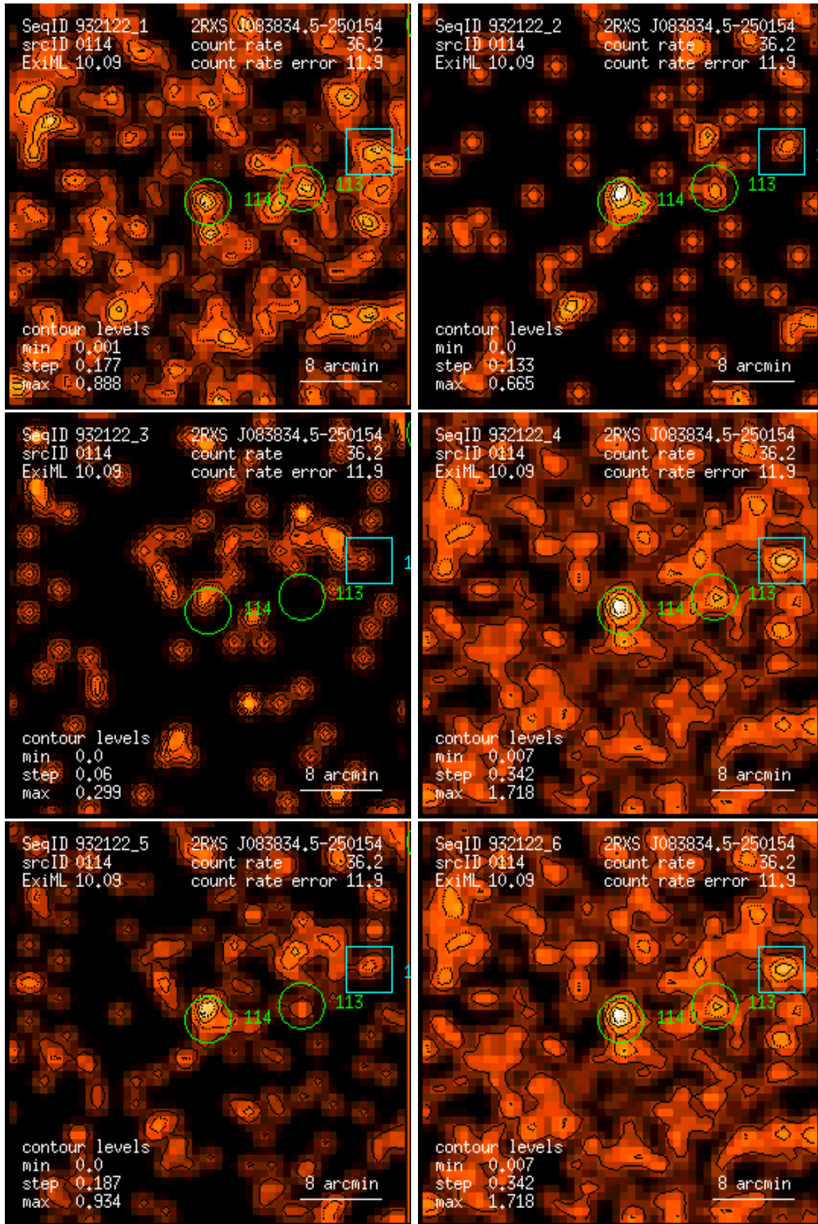
Figure 114: RASS 932122: detection 0114: band rate images, Gaussian filter: (1) PSPC channels 11 – 41, (2) 52 – 90, (3) 91 – 201, (4) 11 – 235, (5) 52 – 201, (6) 11 – 201. Broad band rates in counts/ks. Band rate contour levels in counts/ks/arcmin 2 .
