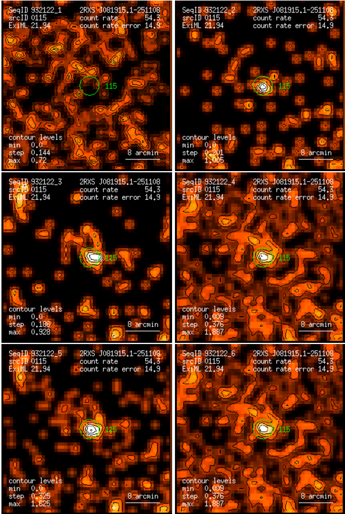
Figure 115: RASS 932122: detection 0115: band rate images, Gaussian filter: (1) PSPC channels 11 – 41, (2) 52 – 90, (3) 91 – 201, (4) 11 – 235, (5) 52 – 201, (6) 11 – 201. Broad band rates in counts/ks. Band rate contour levels in counts/ks/arcmin 2 .
