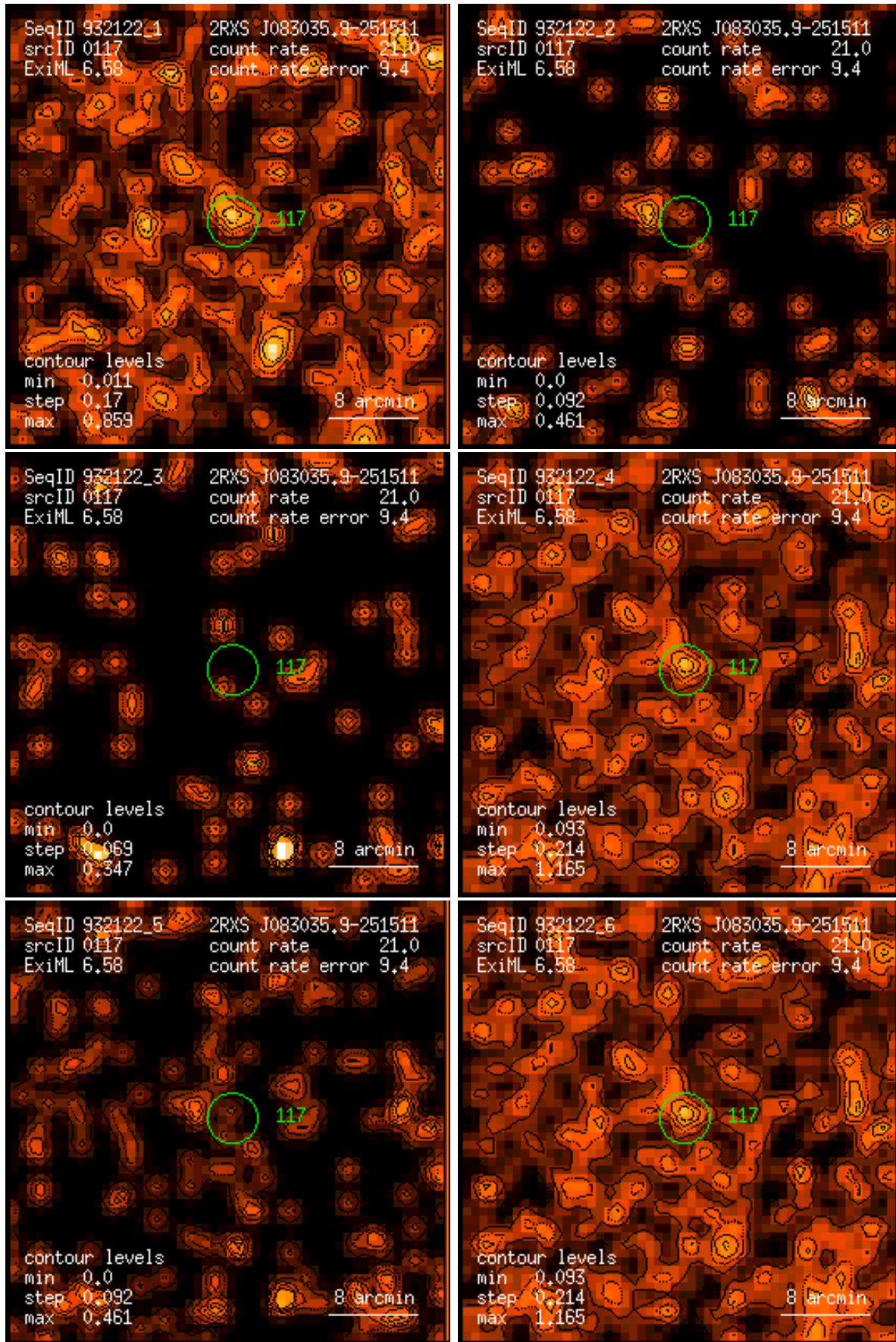
Figure 117: RASS 932122: detection 0117: band rate images, Gaussian filter: (1) PSPC channels 11 – 41, (2) 52 – 90, (3) 91 – 201, (4) 11 – 235, (5) 52 – 201, (6) 11 – 201. Broad band rates in counts/ks. Band rate contour levels in counts/ks/arcmin 2 .
