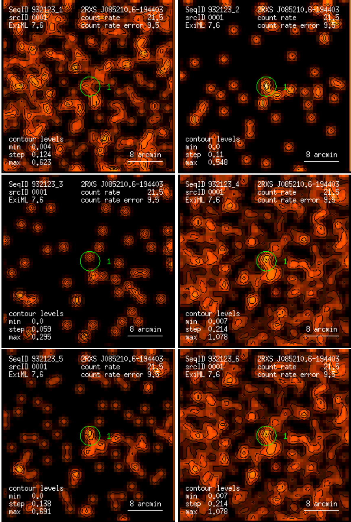
Figure 1: RASS 932123: detection 0001: band rate images, Gaussian filter: (1) PSPC channels 11 – 41, (2) 52 – 90, (3) 91 – 201, (4) 11 – 235, (5) 52 – 201, (6) 11 – 201. Broad band rates in counts/ks. Band rate contour levels in counts/ks/arcmin 2 .
