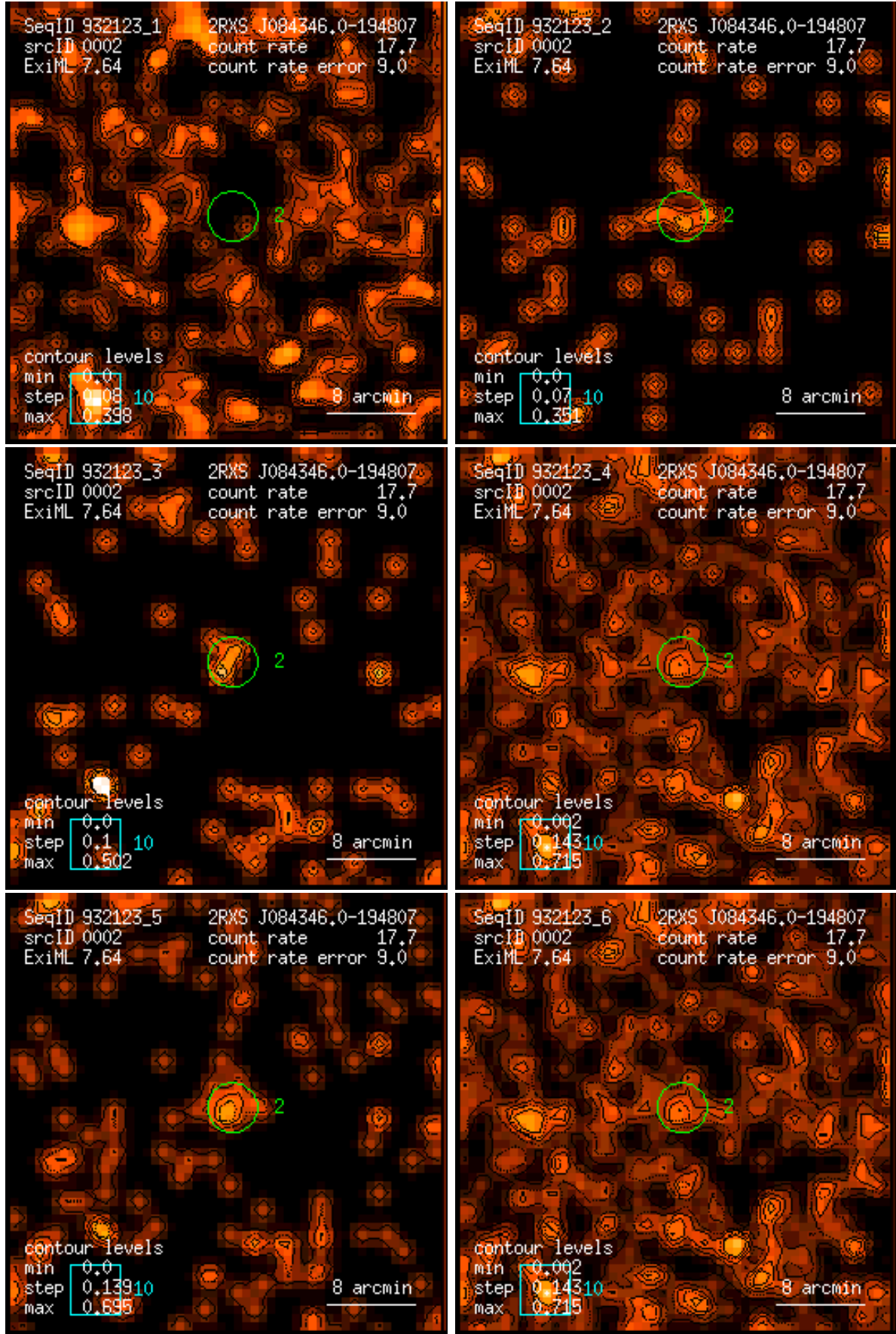
Figure 2: RASS 932123: detection 0002: band rate images, Gaussian filter: (1) PSPC channels 11 – 41, (2) 52 – 90, (3) 91 – 201, (4) 11 – 235, (5) 52 – 201, (6) 11 – 201. Broad band rates in counts/ks. Band rate contour levels in counts/ks/arcmin 2 .
