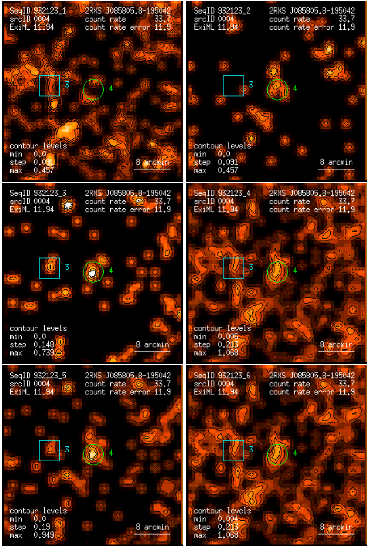
Figure 4: RASS 932123: detection 0004: band rate images, Gaussian filter: (1) PSPC channels 11 – 41, (2) 52 – 90, (3) 91 – 201, (4) 11 – 235, (5) 52 – 201, (6) 11 – 201. Broad band rates in counts/ks. Band rate contour levels in counts/ks/arcmin 2 .
