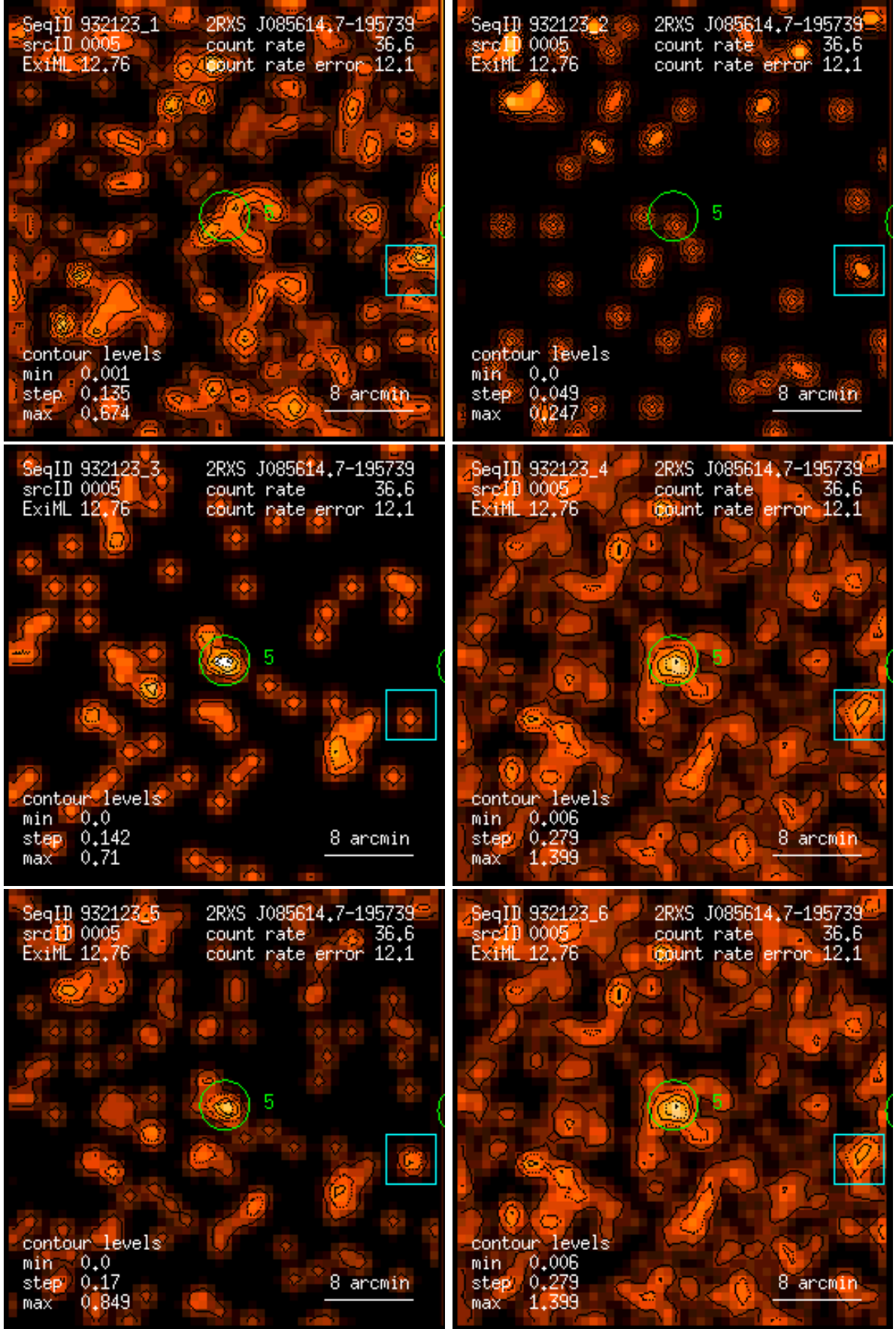
Figure 5: RASS 932123: detection 0005: band rate images, Gaussian filter: (1) PSPC channels 11 – 41, (2) 52 – 90, (3) 91 – 201, (4) 11 – 235, (5) 52 – 201, (6) 11 – 201. Broad band rates in counts/ks. Band rate contour levels in counts/ks/arcmin 2 .
