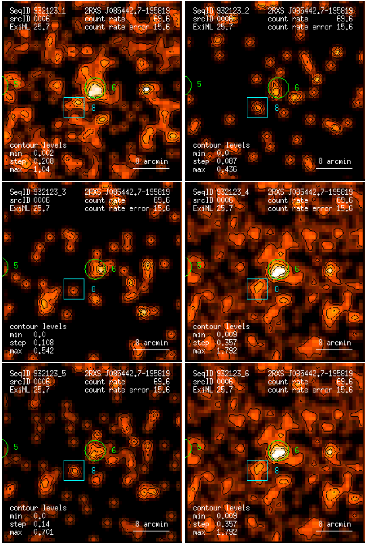
Figure 6: RASS 932123: detection 0006: band rate images, Gaussian filter: (1) PSPC channels 11 – 41, (2) 52 – 90, (3) 91 – 201, (4) 11 – 235, (5) 52 – 201, (6) 11 – 201. Broad band rates in counts/ks. Band rate contour levels in counts/ks/arcmin 2 .
