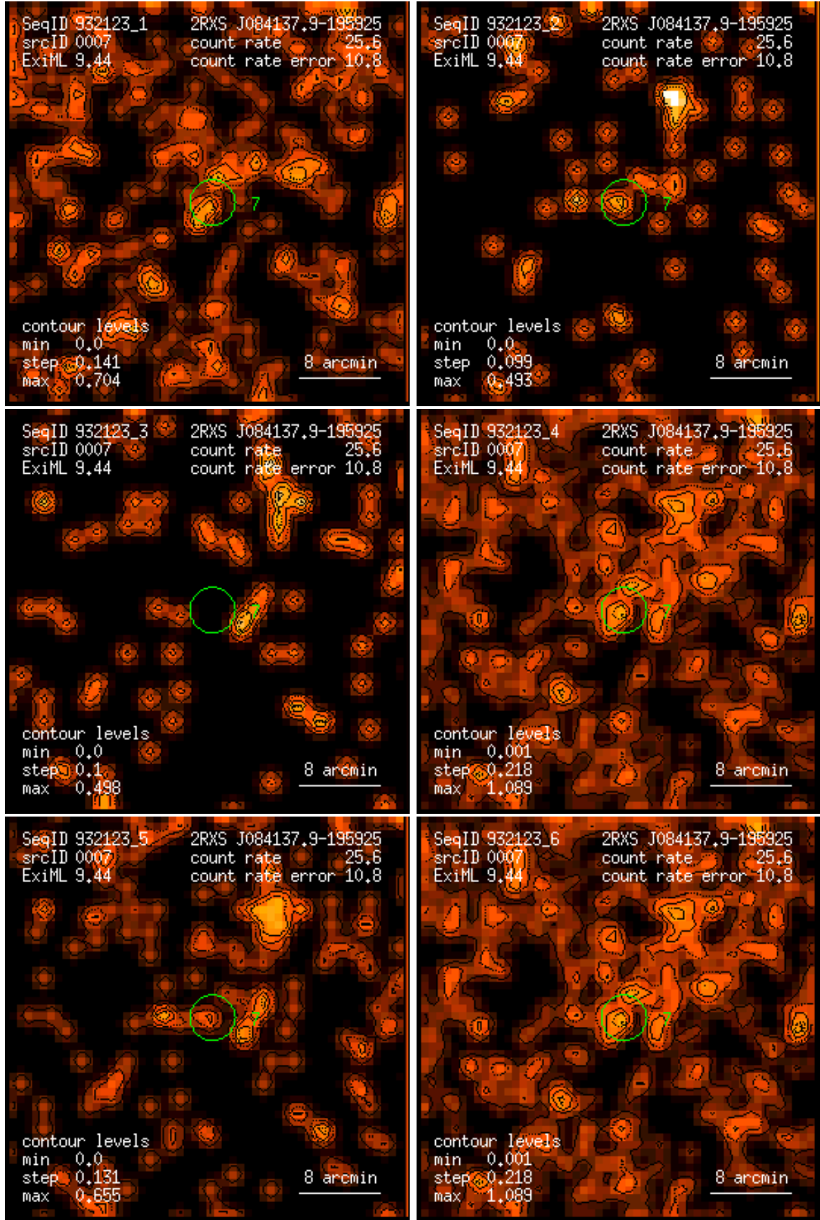
Figure 7: RASS 932123: detection 0007: band rate images, Gaussian filter: (1) PSPC channels 11 – 41, (2) 52 – 90, (3) 91 – 201, (4) 11 – 235, (5) 52 – 201, (6) 11 – 201. Broad band rates in counts/ks. Band rate contour levels in counts/ks/arcmin 2 .
