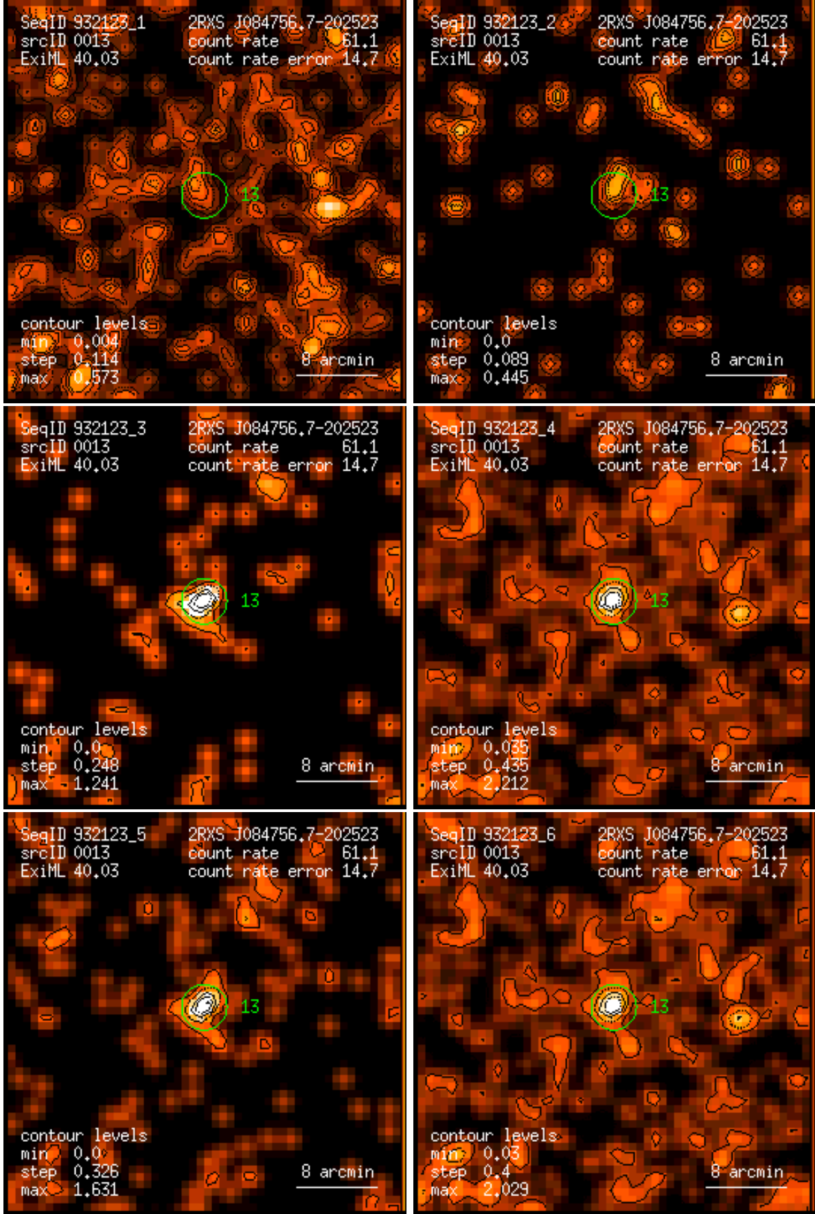
Figure 13: RASS 932123: detection 0013: band rate images, Gaussian filter: (1) PSPC channels 11 – 41, (2) 52 – 90, (3) 91 – 201, (4) 11 – 235, (5) 52 – 201, (6) 11 – 201. Broad band rates in counts/ks. Band rate contour levels in counts/ks/arcmin 2 .
