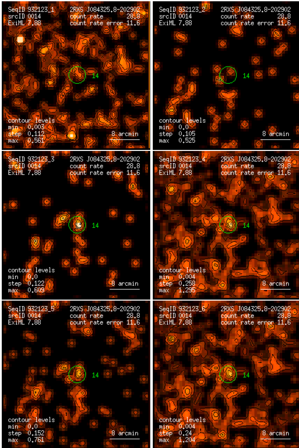
Figure 14: RASS 932123: detection 0014: band rate images, Gaussian filter: (1) PSPC channels 11 – 41, (2) 52 – 90, (3) 91 – 201, (4) 11 – 235, (5) 52 – 201, (6) 11 – 201. Broad band rates in counts/ks. Band rate contour levels in counts/ks/arcmin 2 .
