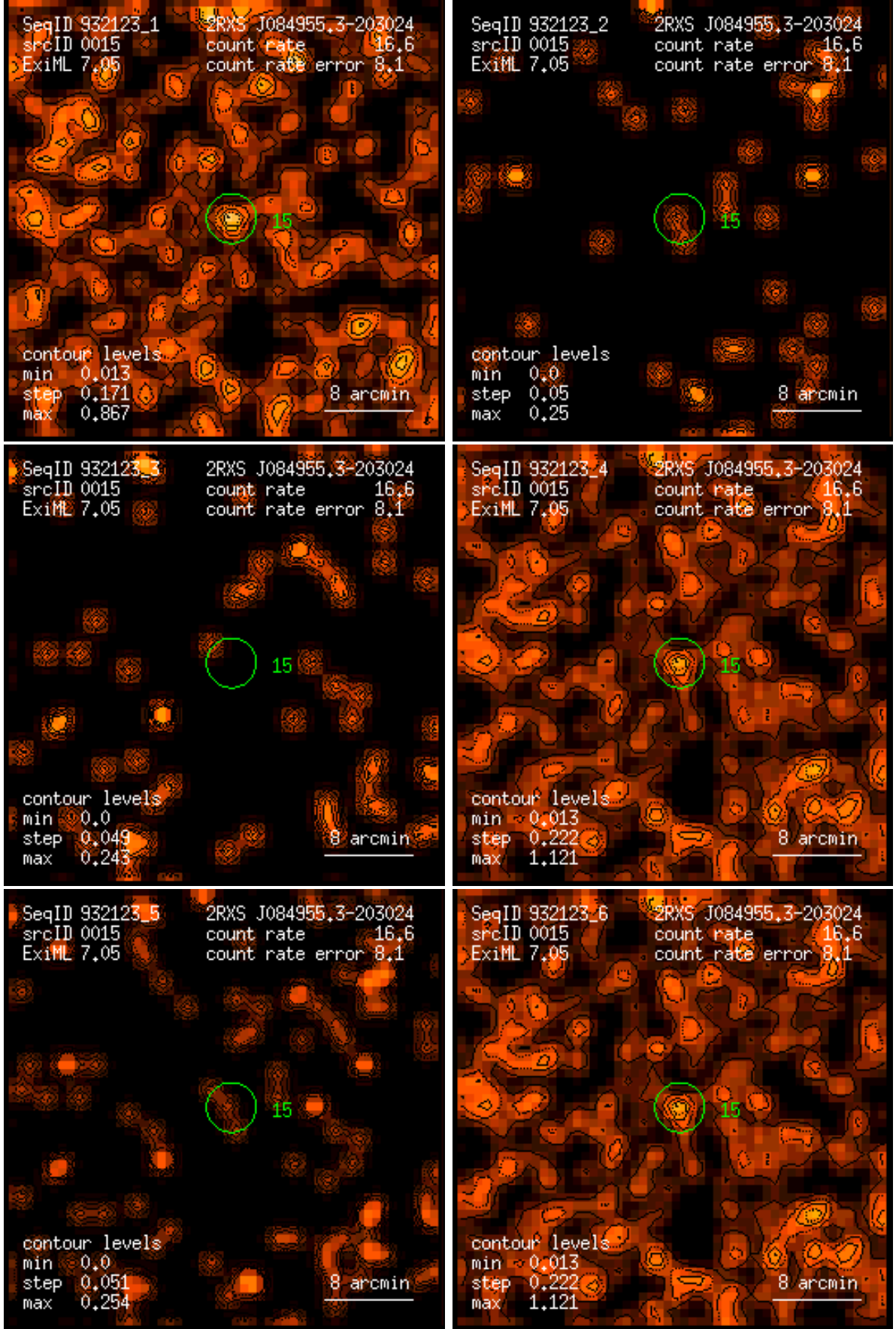
Figure 15: RASS 932123: detection 0015: band rate images, Gaussian filter: (1) PSPC channels 11 – 41, (2) 52 – 90, (3) 91 – 201, (4) 11 – 235, (5) 52 – 201, (6) 11 – 201. Broad band rates in counts/ks. Band rate contour levels in counts/ks/arcmin 2 .
