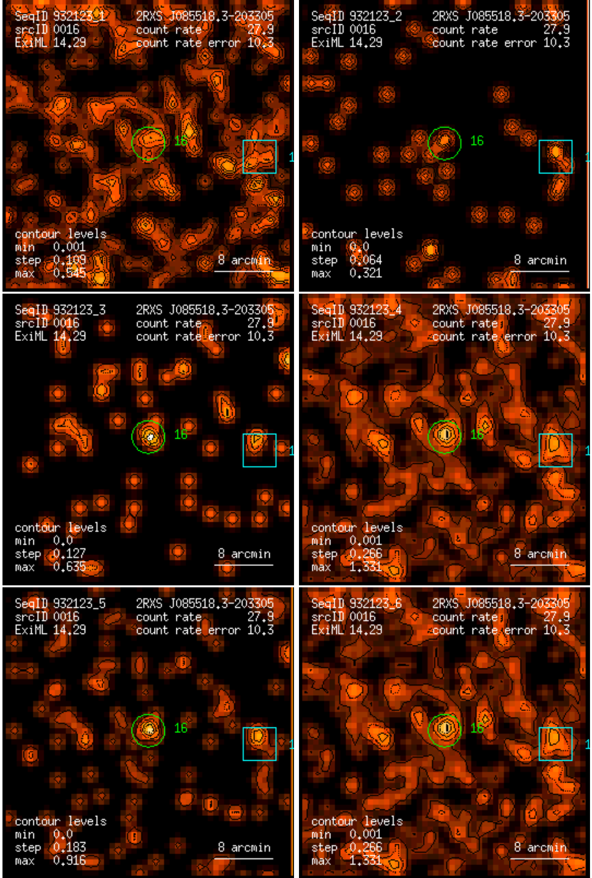
Figure 16: RASS 932123: detection 0016: band rate images, Gaussian filter: (1) PSPC channels 11 – 41, (2) 52 – 90, (3) 91 – 201, (4) 11 – 235, (5) 52 – 201, (6) 11 – 201. Broad band rates in counts/ks. Band rate contour levels in counts/ks/arcmin 2 .
