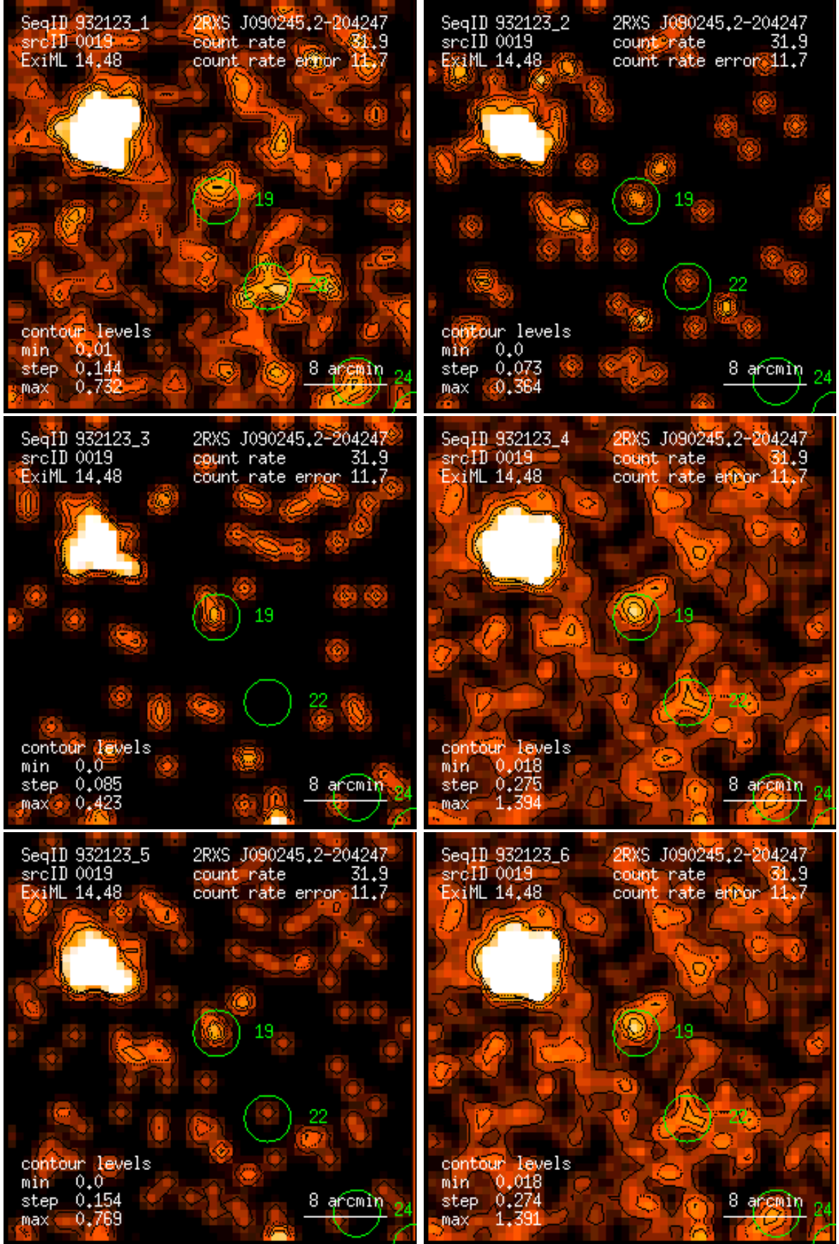
Figure 19: RASS 932123: detection 0019: band rate images, Gaussian filter: (1) PSPC channels 11 – 41, (2) 52 – 90, (3) 91 – 201, (4) 11 – 235, (5) 52 – 201, (6) 11 – 201. Broad band rates in counts/ks. Band rate contour levels in counts/ks/arcmin 2 .
